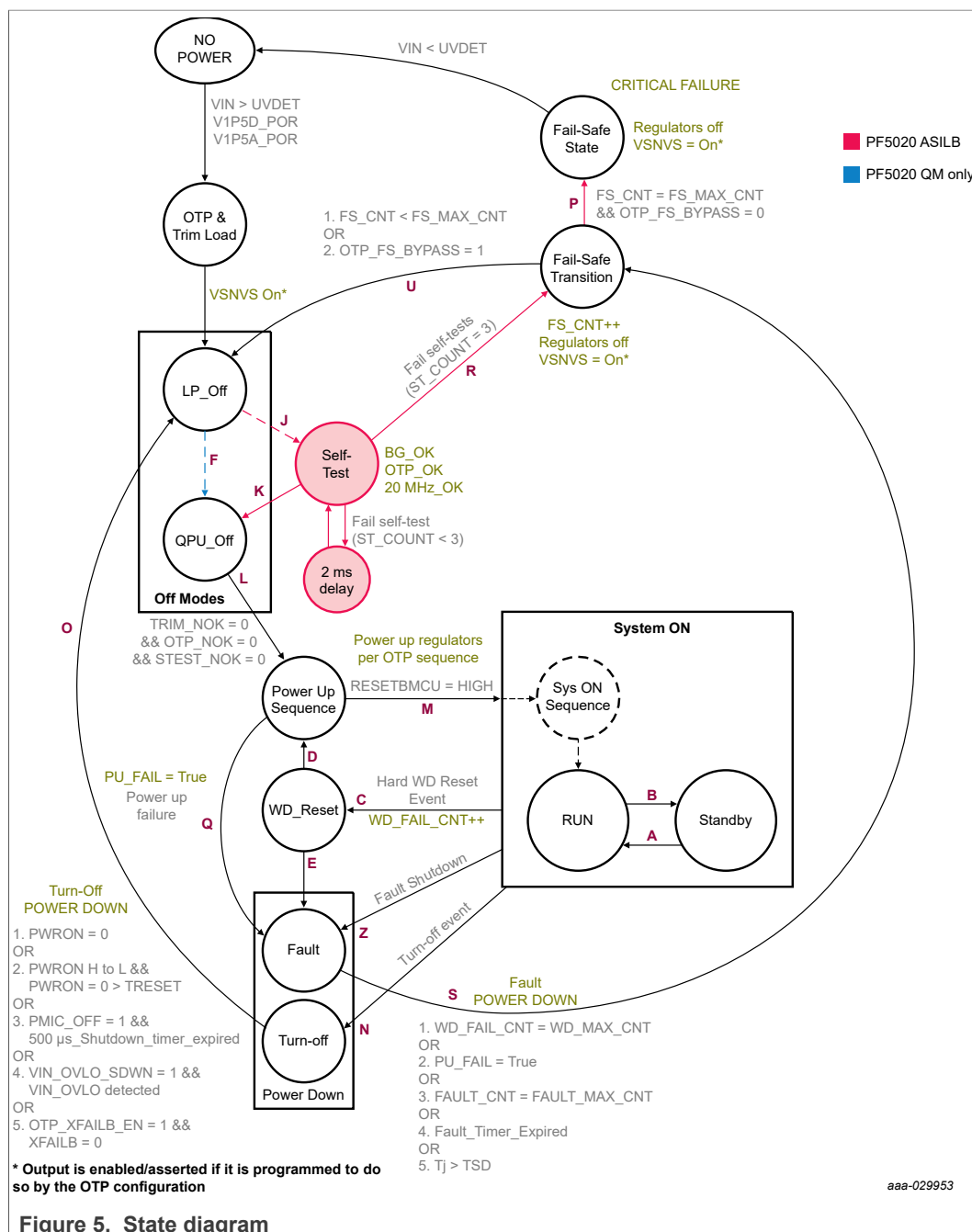
Figure 5. State diagram
