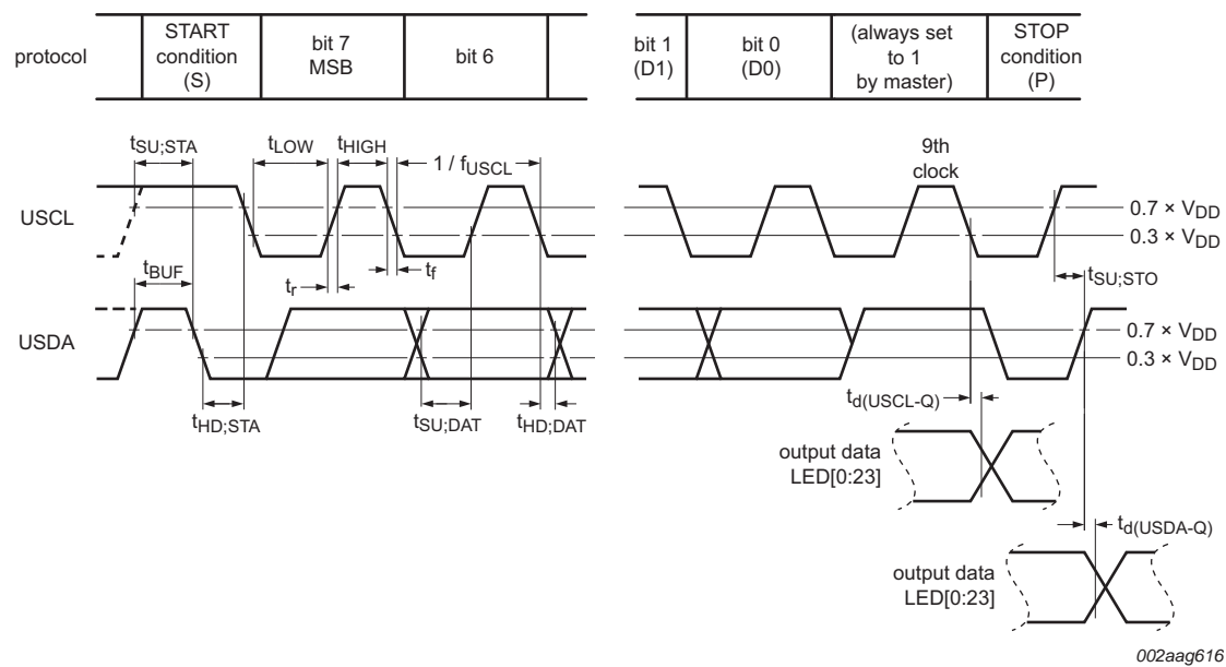
Fig 16. U 2 Fm I 2 C-bus timing and output timing diagram
