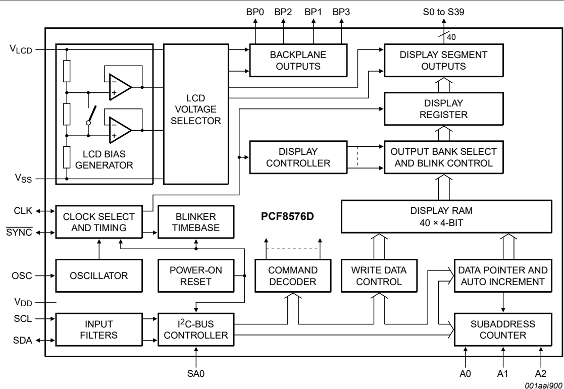
Figure 1. Block diagram of PCF8576D
