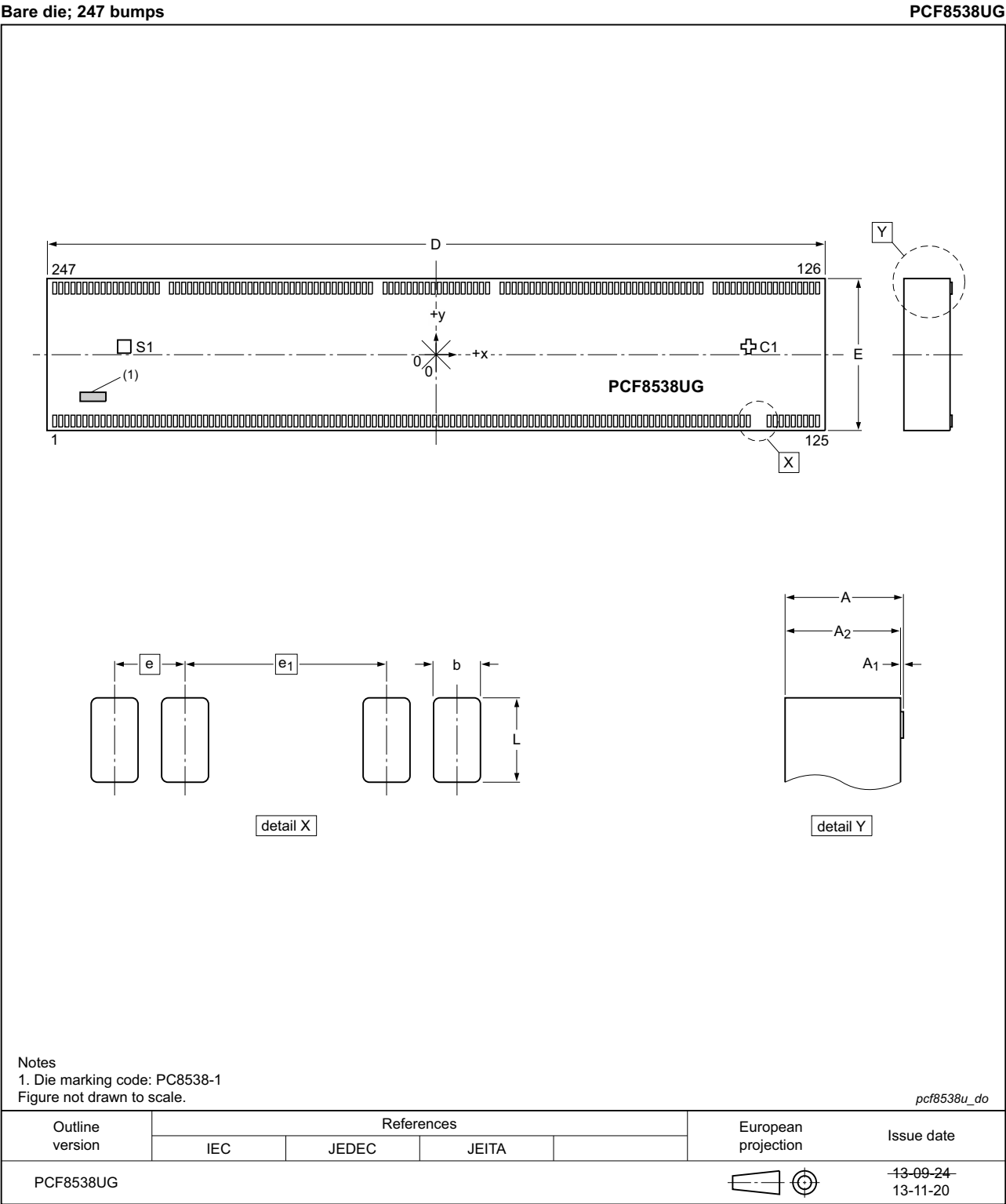
Fig 64. Bare die outline of PCF8538UG
