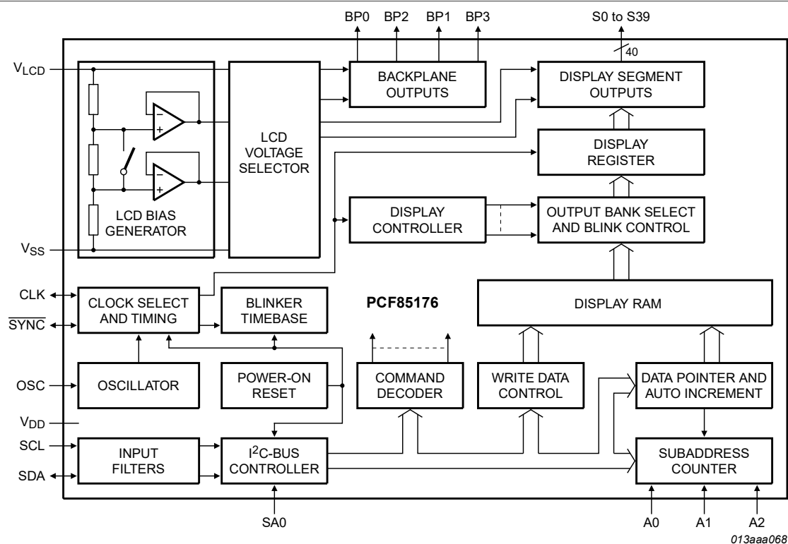
Figure 1. Block diagram of PCF85176
