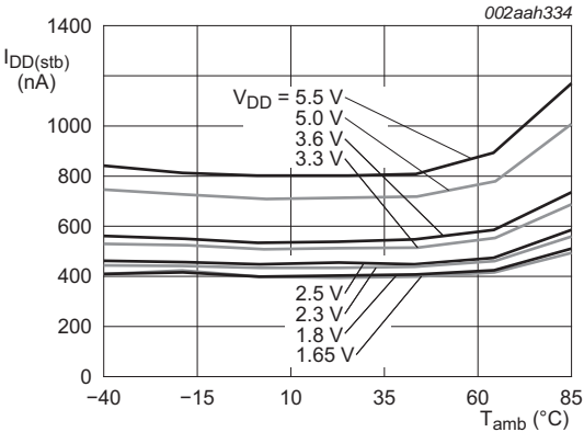
Fig 22. Standby supply current versus ambient temperature
