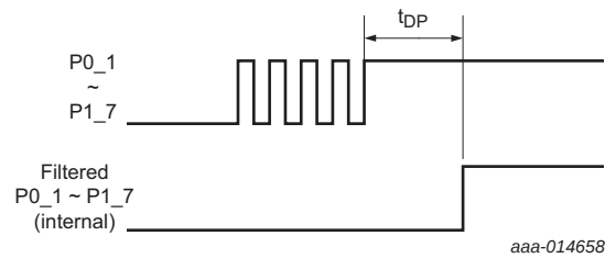
Fig 14. Switch debounce timing
