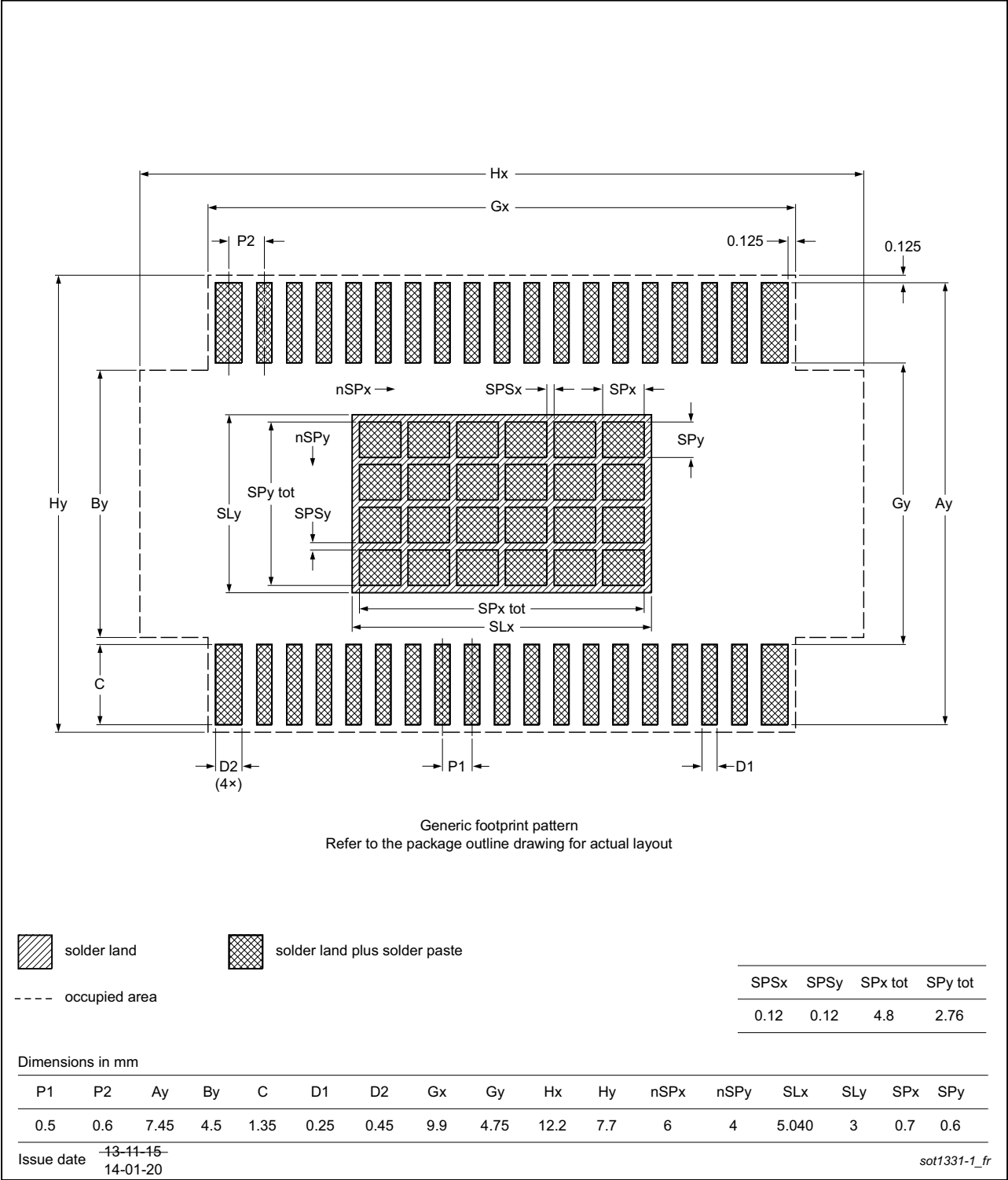
Footprint information for reflow soldering of HTSSOP38 package
