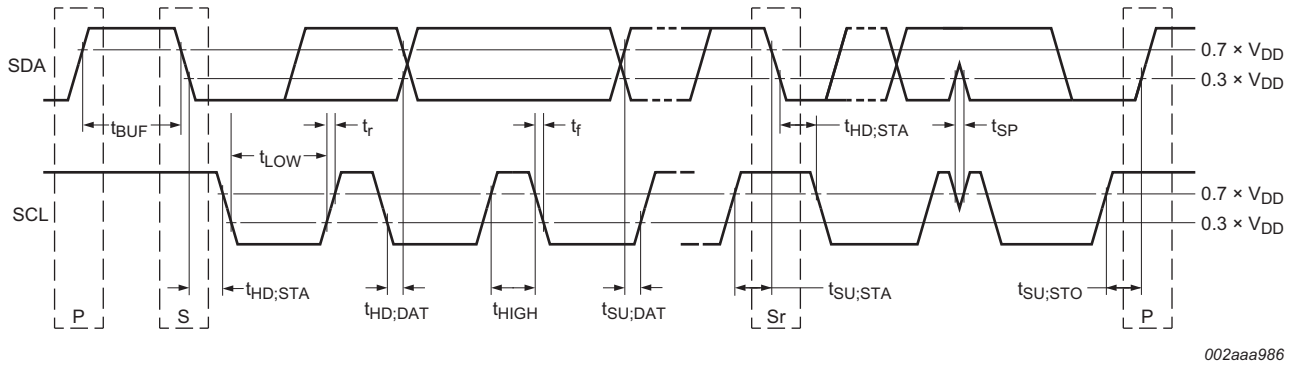
Fig 21. Definition of timing
