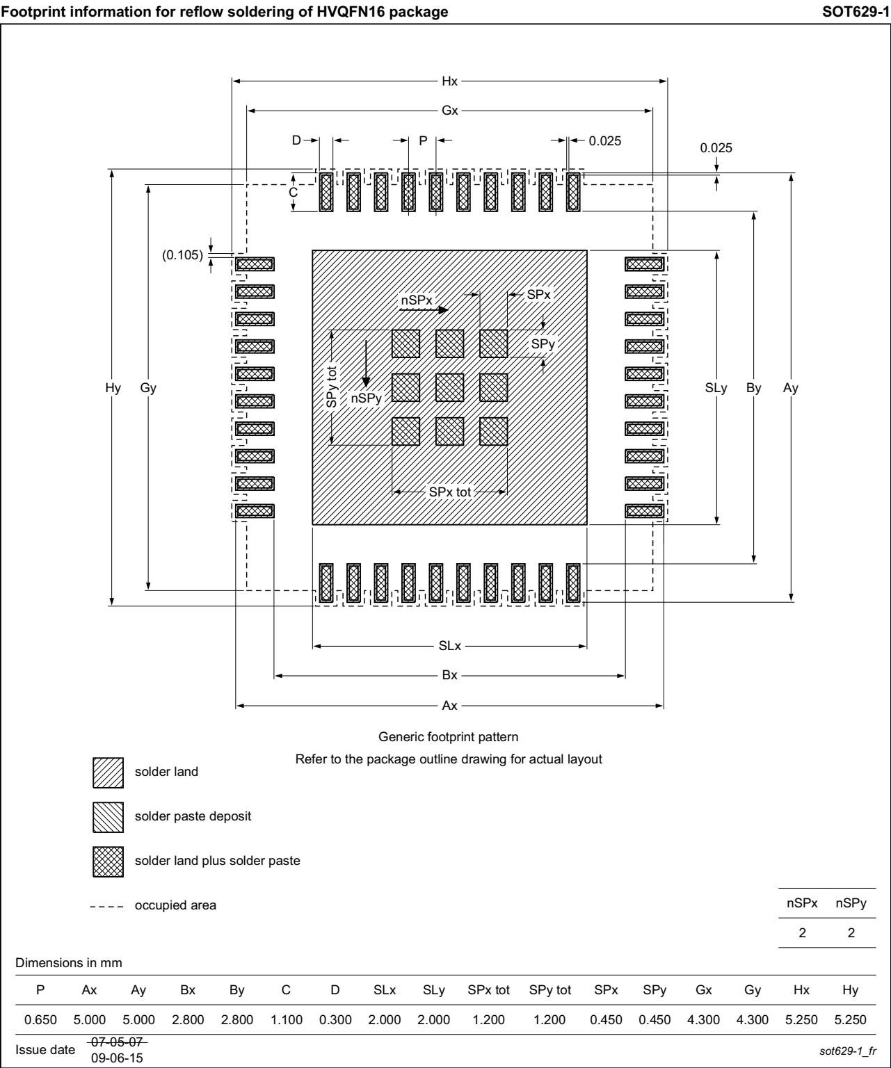
Fig 25. PCB footprint for SOT629-1 (HVQFN16); reflow soldering
