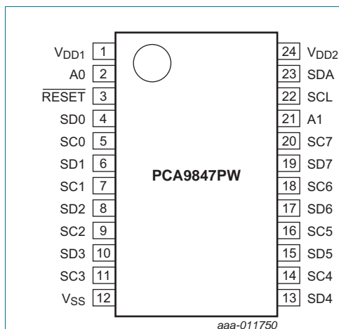
Fig 2. Pin configuration for TSSOP24
