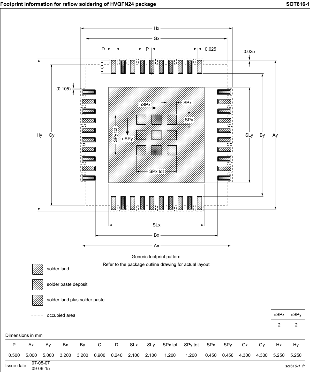
Fig 25. PCB footprint for SOT616-1 (HVQFN24); reflow soldering
