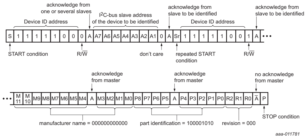
Fig 9. Device ID field read operation
