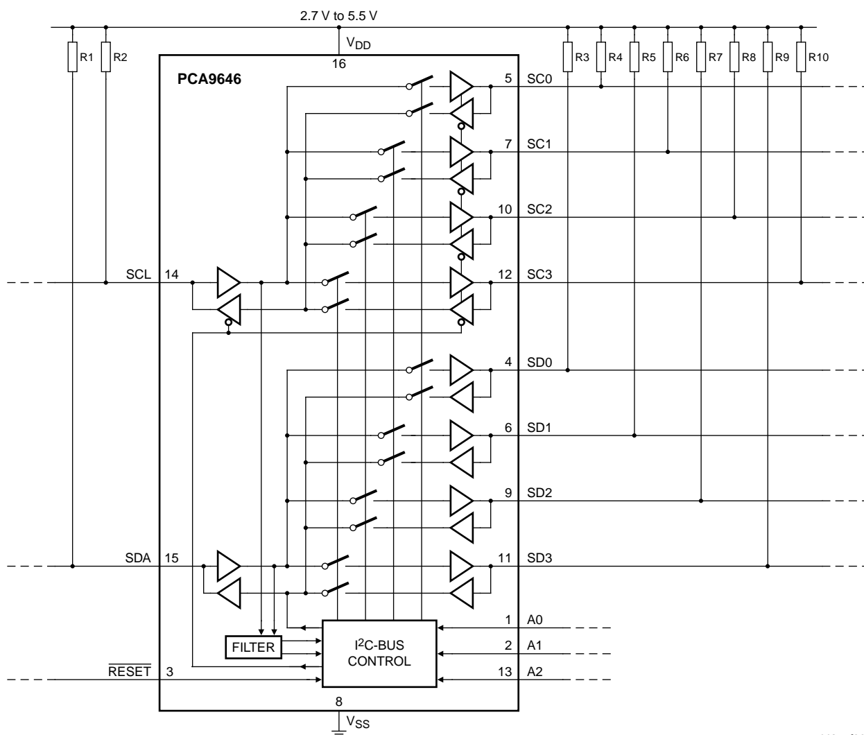
Fig 1. Simplified block diagram of PCA9646
