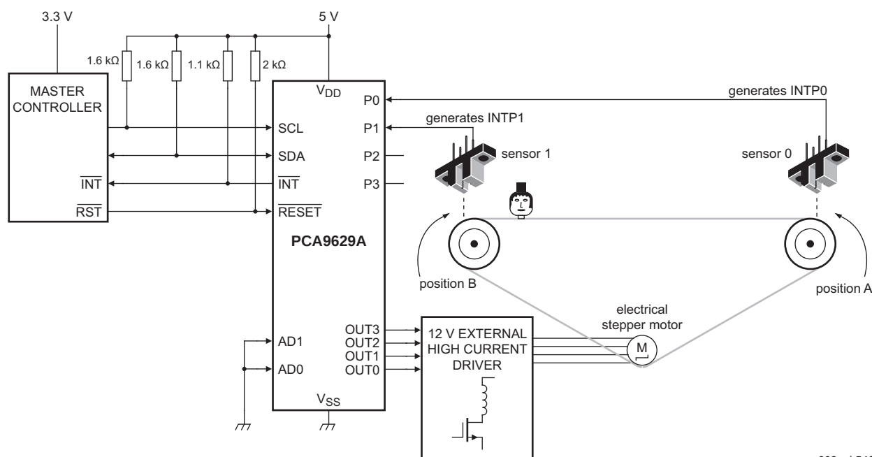
Fig 23. Typical application
