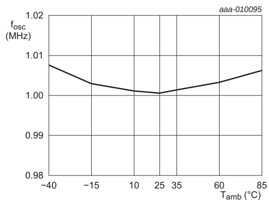
Fig 28. Typical oscillator frequency versus temperature
