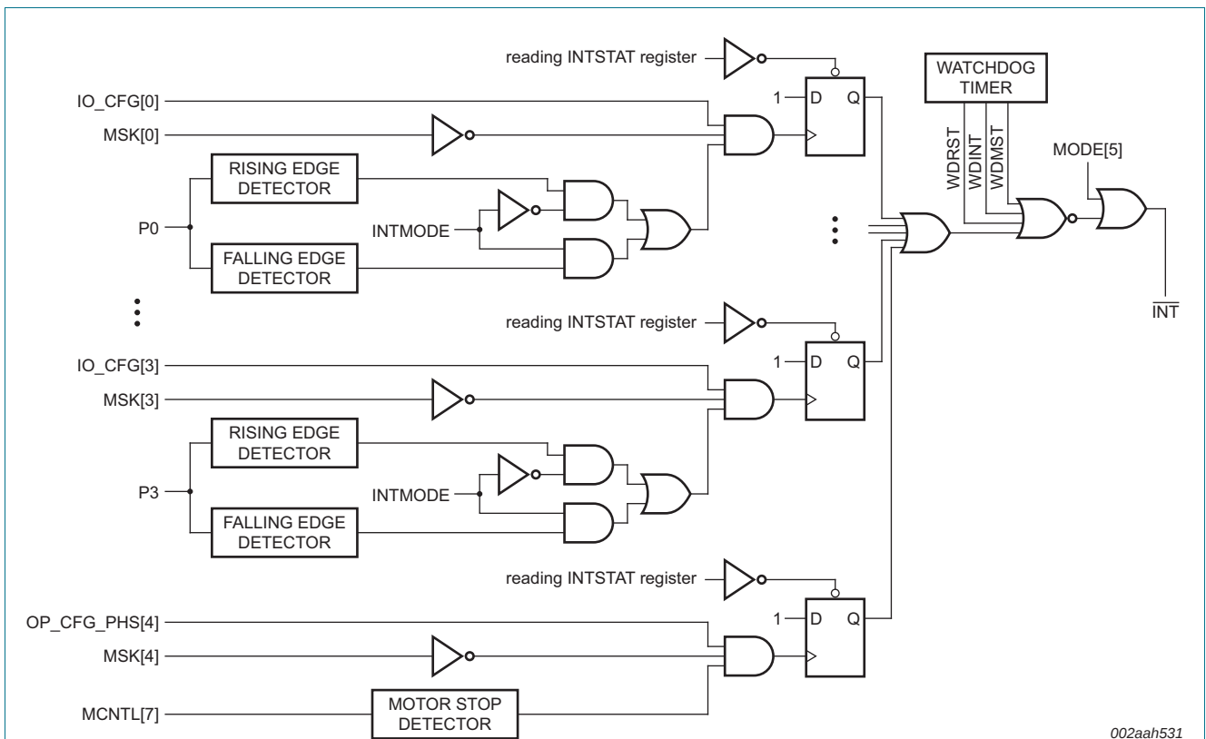
Fig 6. PCA9629A interrupt logic
