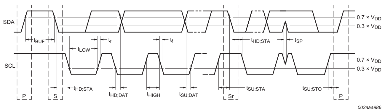
Fig 26. Definition of timing
