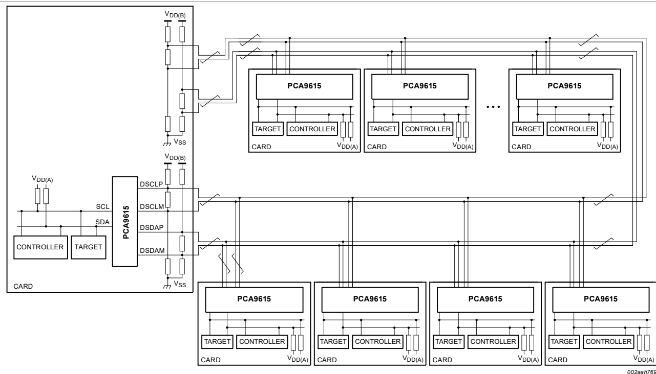
Figure 9. PCA9615 application diagram; V DD and V SS are not routed through the cable
