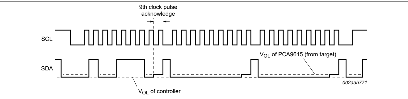
Figure 12. Single-ended bus waveform (controller side of bus)
