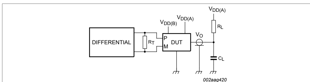
Figure 14. Test circuit for differential outputs
