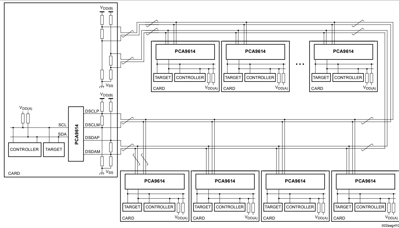
Figure 8. PCA9614 application diagram; V DD and V SS are not routed through the cable
