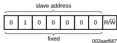
Fig 6. PCA9575 device address for 24-pin version
