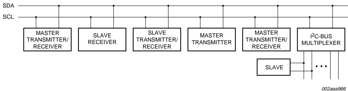
Fig 7. System configuration
