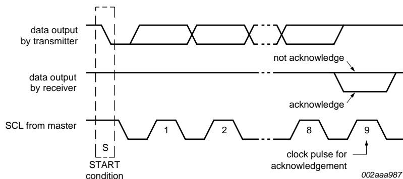
Fig 8. Acknowledgement on the I 2 C-bus
