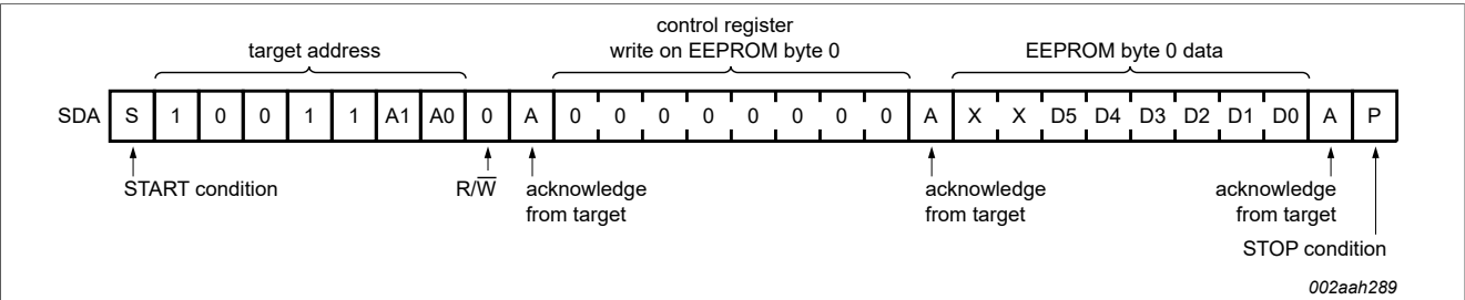
Figure 9. Write on one EEPROM, assuming WP = 0
