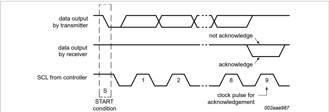
Figure 8. Acknowledgement on the I 2 C-bus
