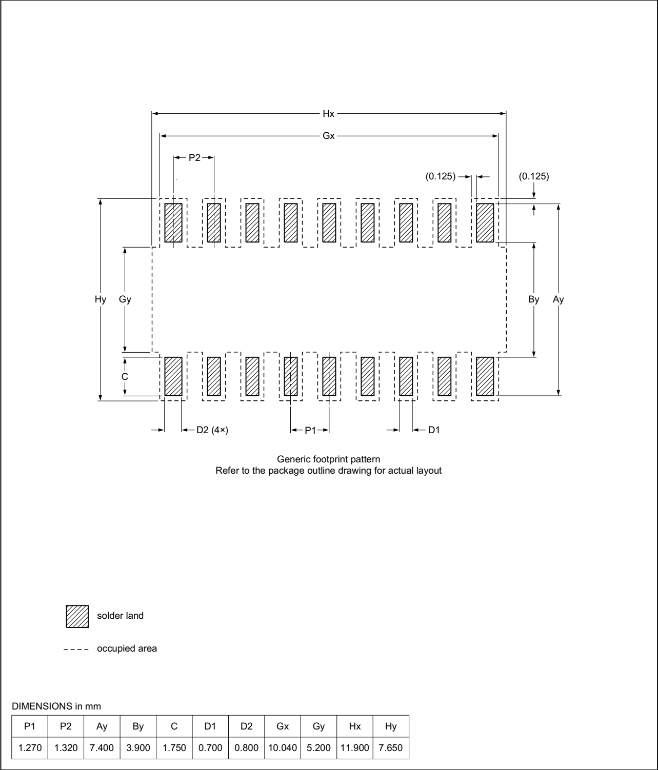
Footprint information for reflow soldering of SO16 package
