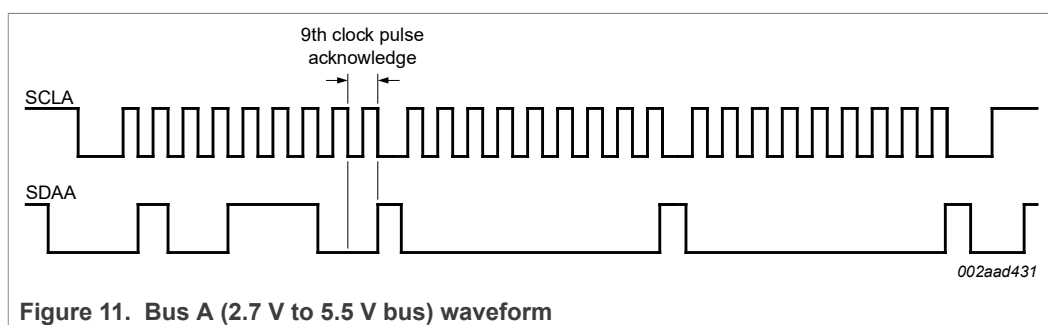
Figure 11. Bus A (2.7 V to 5.5 V bus) waveform
