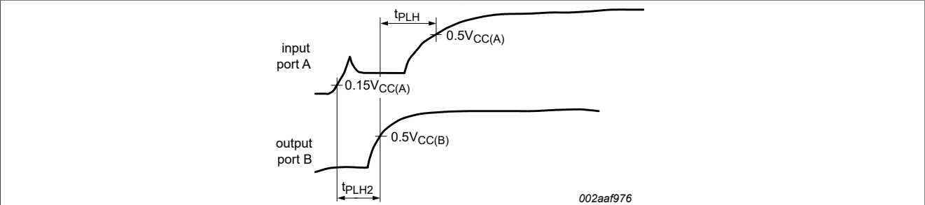
Figure 9. Propagation delay from the port A's external driver switching off to port B LOW-to-HIGH transition; port A to port B
