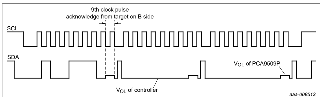
Figure 6. Bus A lower voltage waveform
