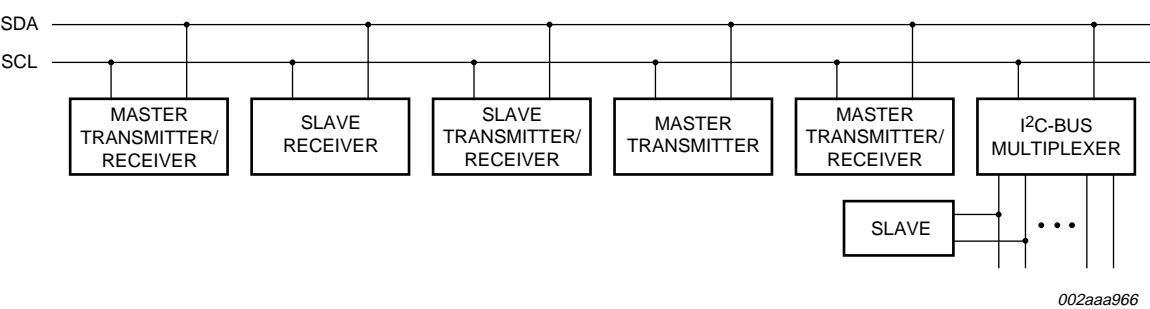
Fig 17. System configuration
