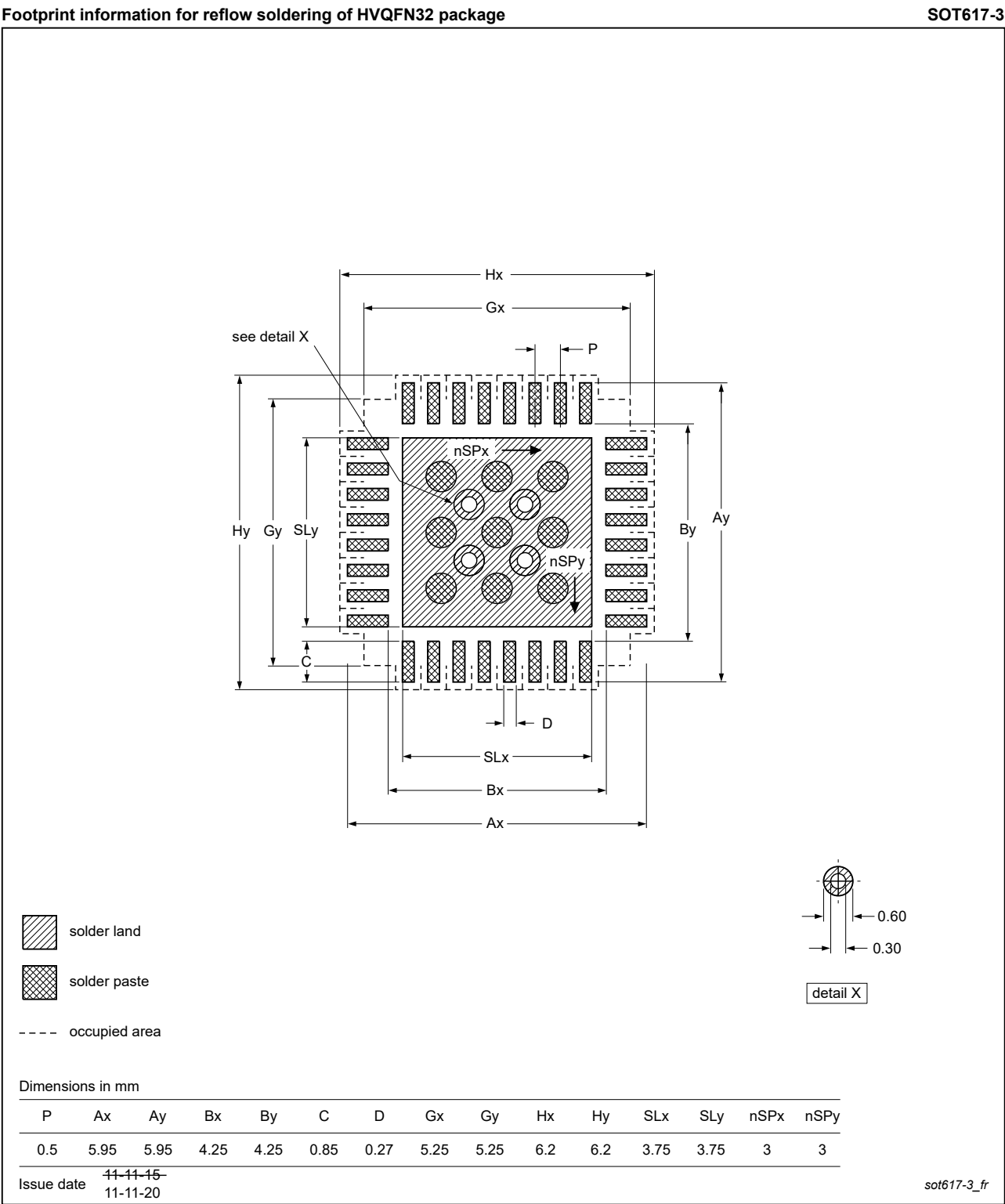
Figure 32. Footprint information for reflow soldering of SOT617-3 (HVQFN32) of PCA8561
