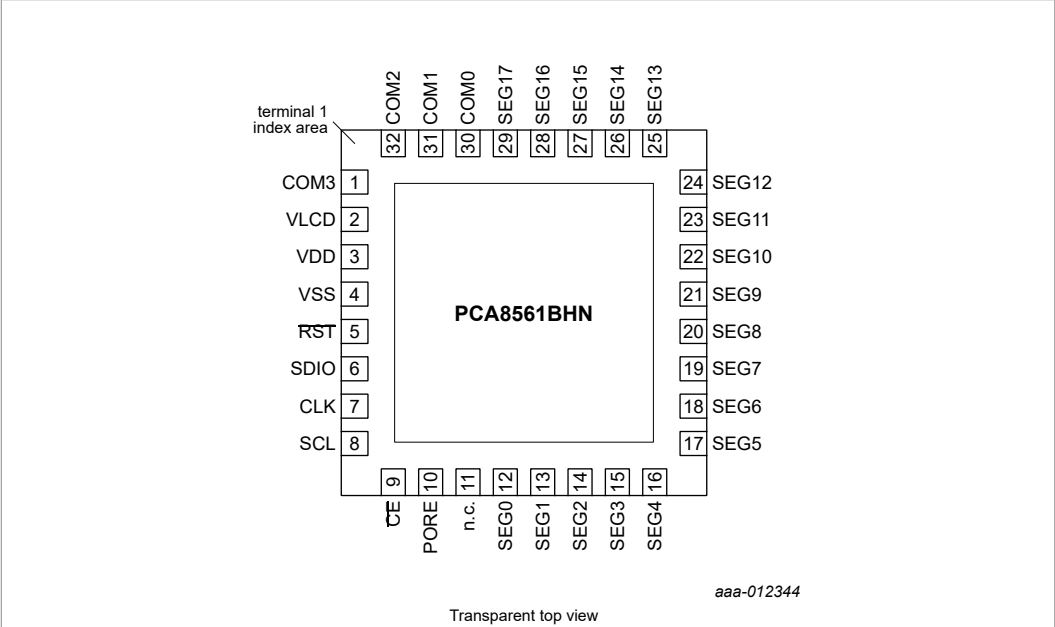
For mechanical details, see Figure 30 . Figure 4. Pin configuration of PCA8561BHN (HVQFN32)
