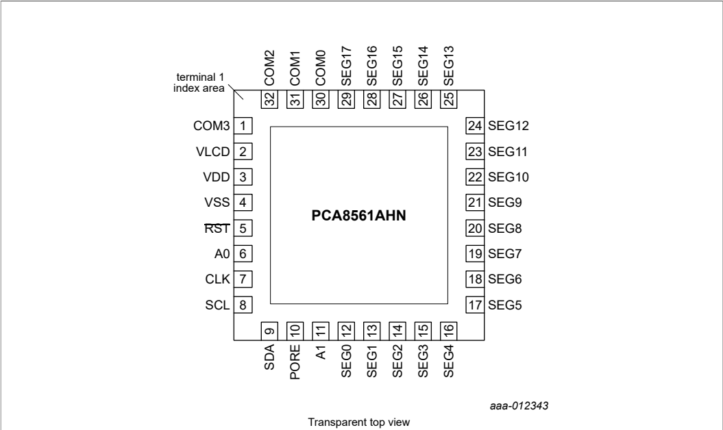
For mechanical details, see Figure 30 . Figure 3. Pin configuration of PCA8561AHN (HVQFN32)
