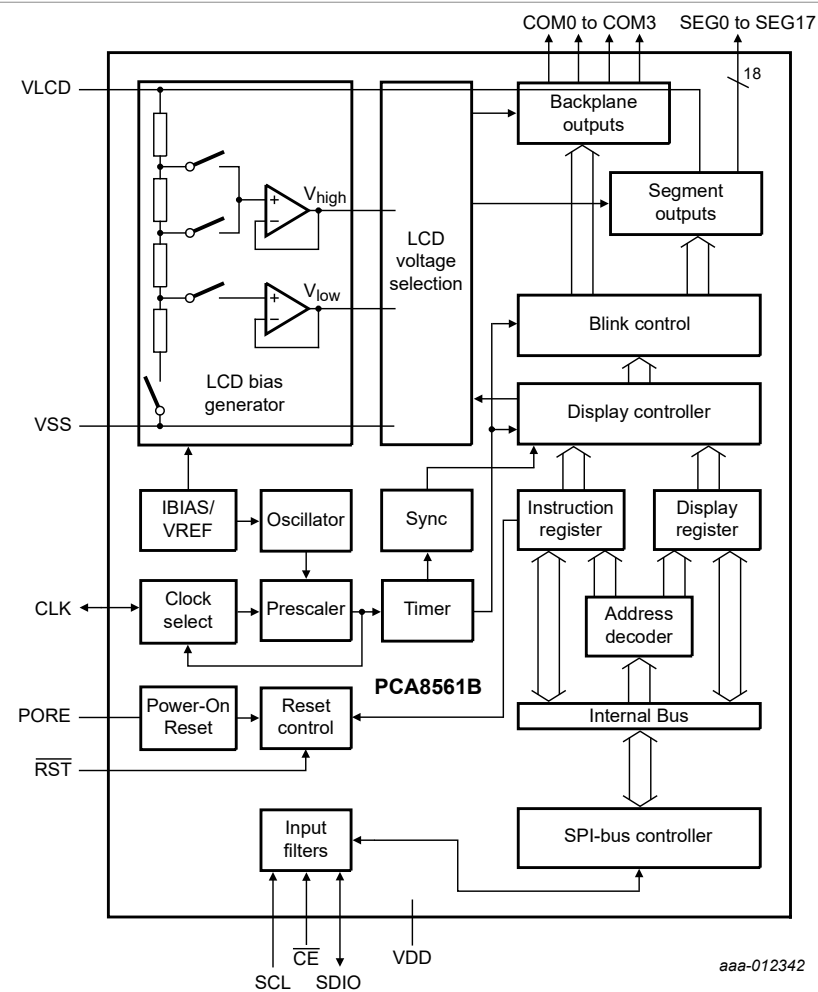
Figure 2. Block diagram of PCA8561B
