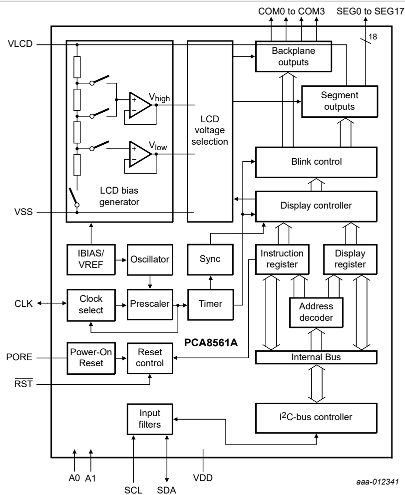
Figure 1. Block diagram of PCA8561A
