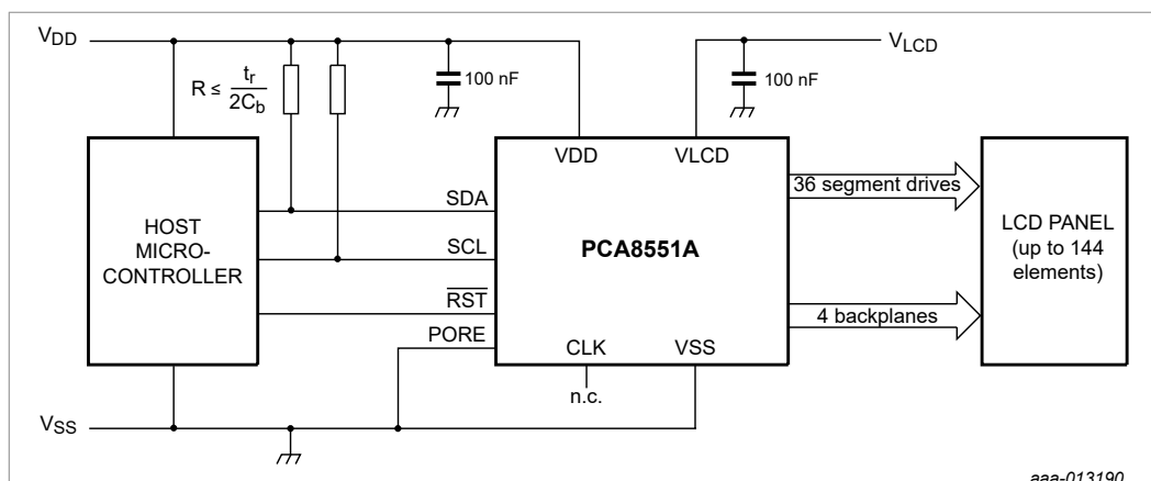
Figure 9. Typical system configuration using I 2 C-bus, internal power-on reset disabled
