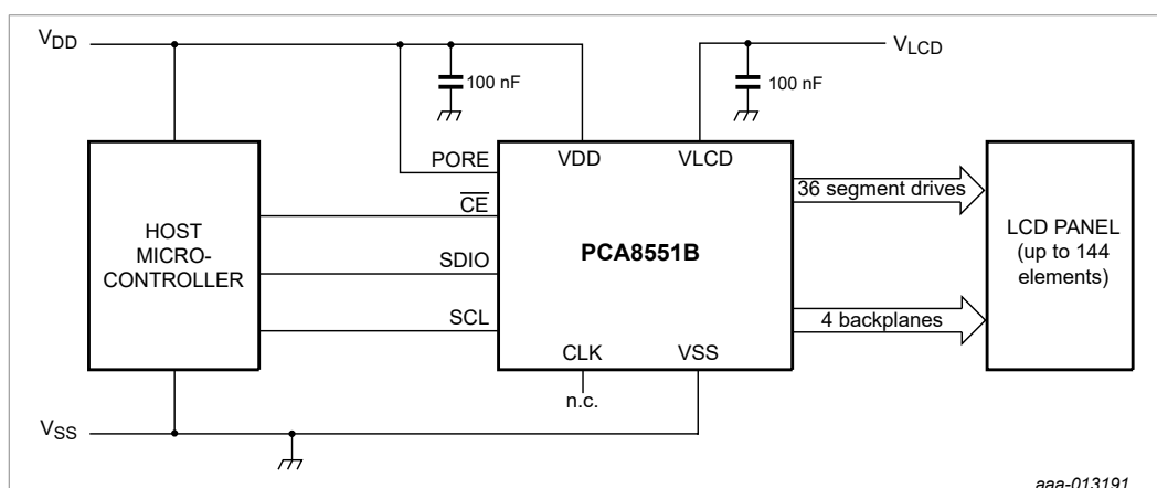
Figure 10. Typical system configuration using SPI-bus, internal power-on reset enabled
