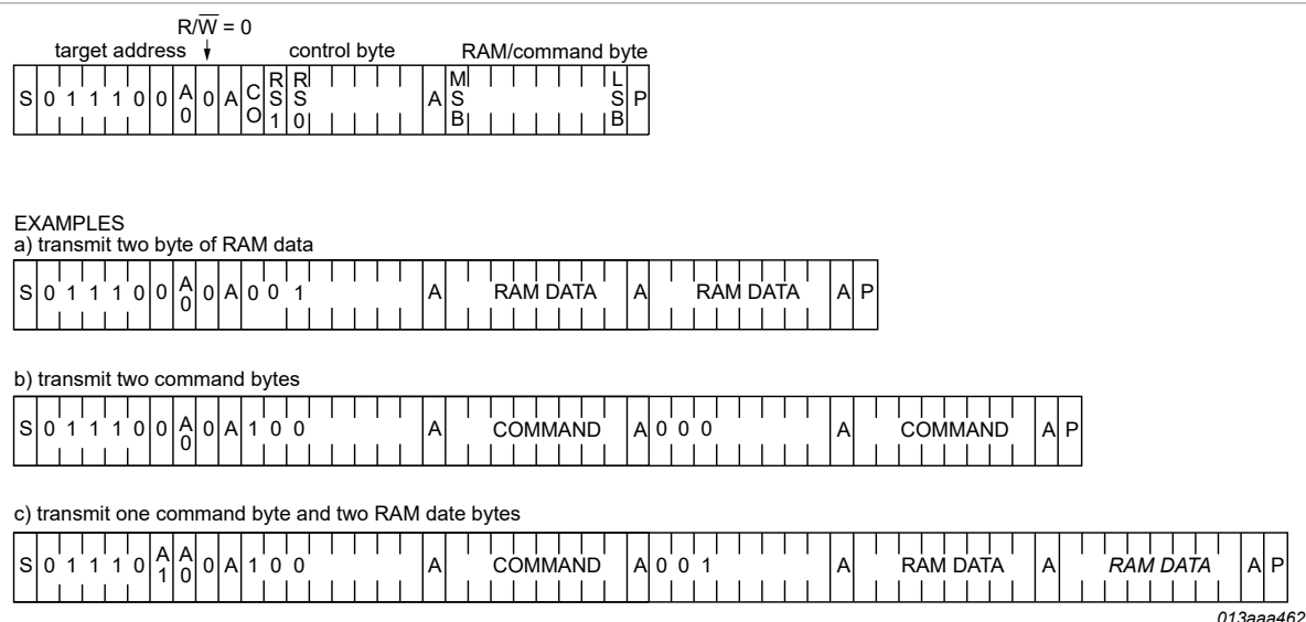
Figure 36. I 2 C-bus protocol write mode
