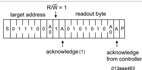
Figure 37. I 2 C-bus protocol read mode
