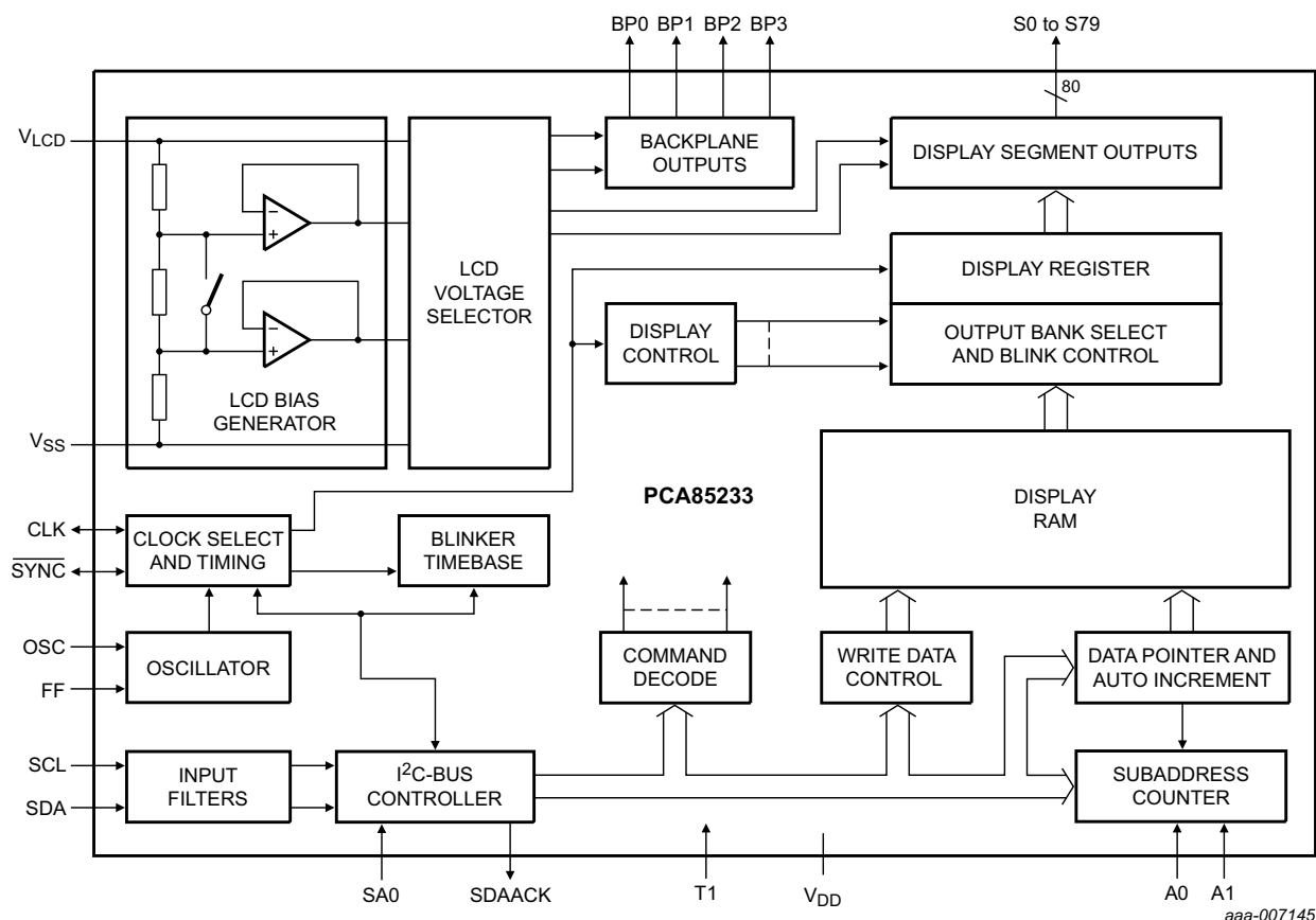
Fig 2. Block diagram of PCA85233
