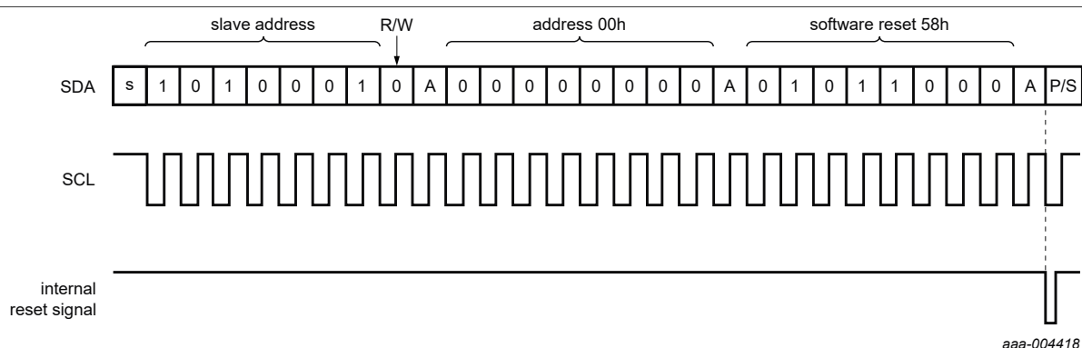
Figure 6. Software reset command
