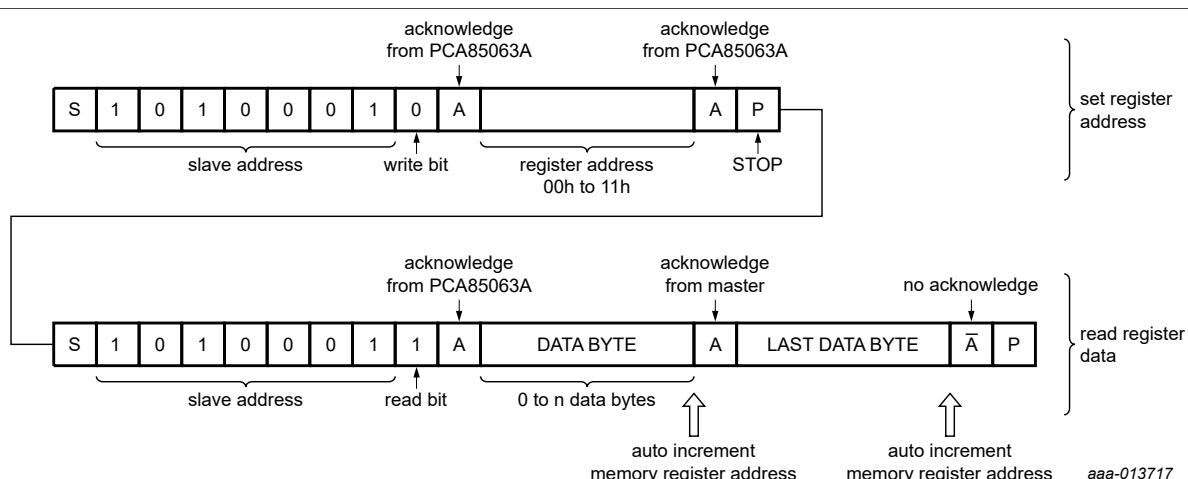
Figure 21. Master reads after setting register address (write register address; READ data)
