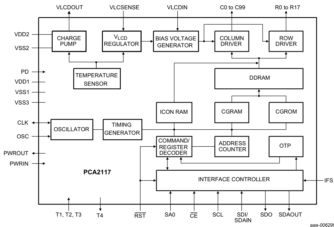
Fig 1. Block diagram of PCA2117
