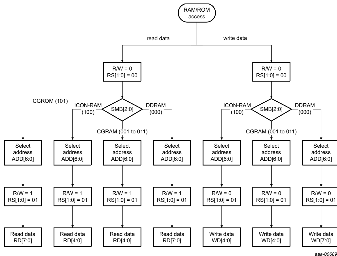
Fig 31. RAM/ROM access flowchart
