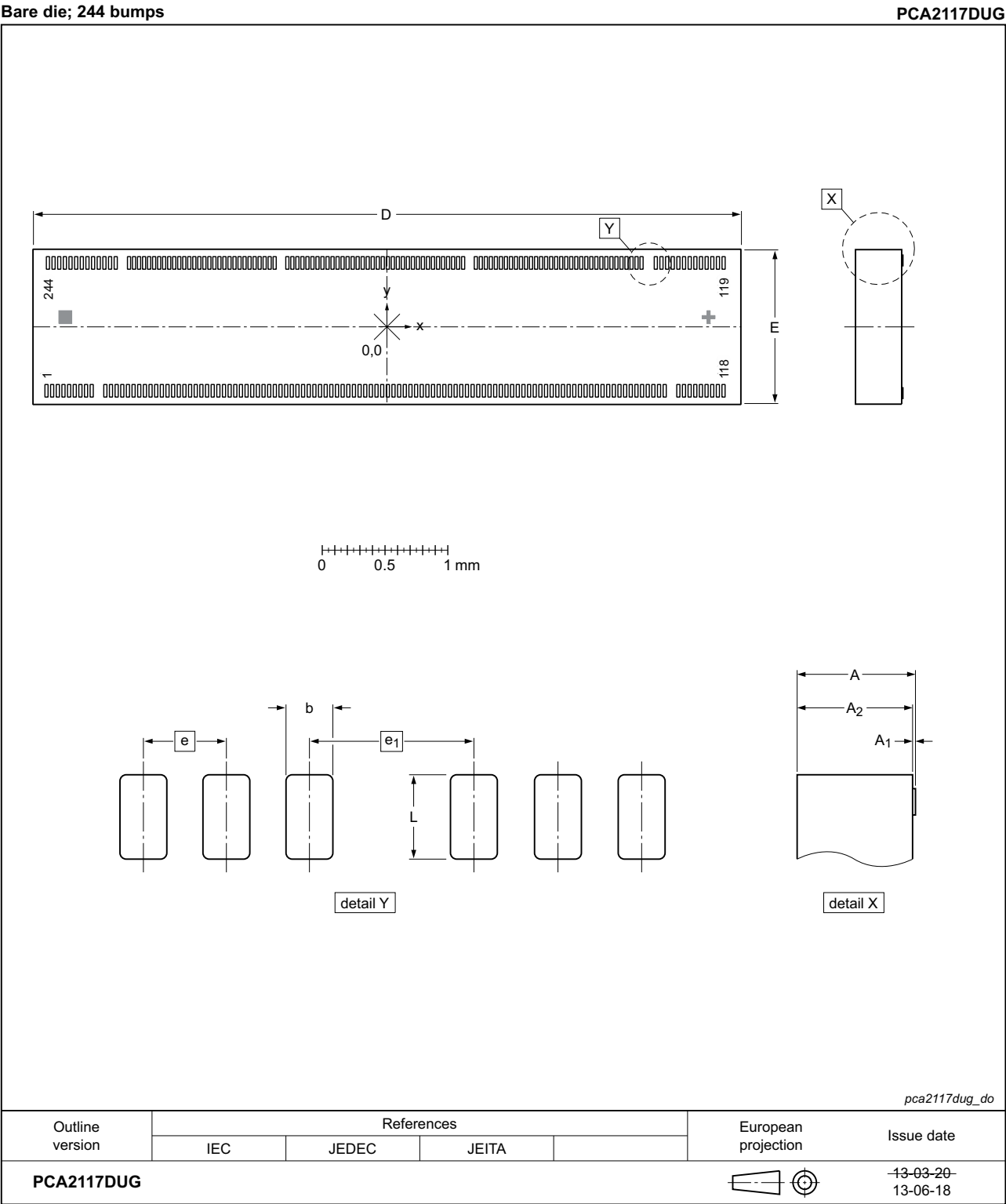
Fig 61. Bare die outline of PCA2117DUGx
