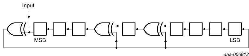
Fig 32. Logic diagram of the CRC8 generator
