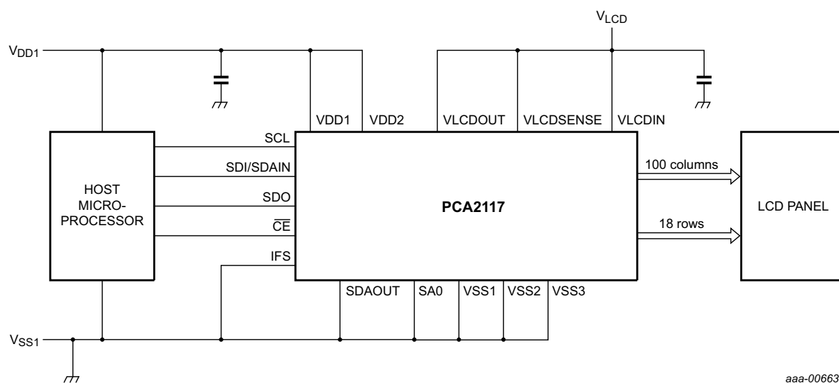
Fig 17. Typical system configuration if using the external V_{LCD} and SPI-bus
