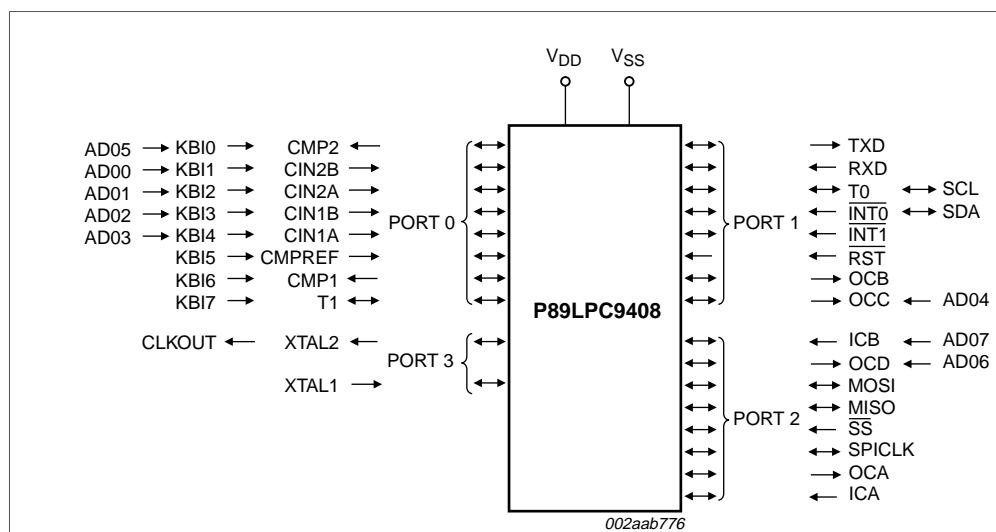
Fig 4. P89LPC9408 functional diagram
