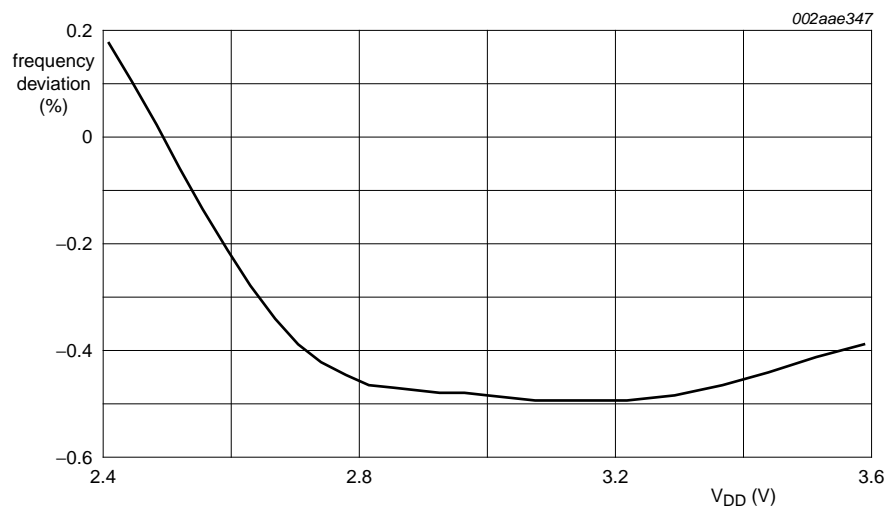
Fig 36. Average internal RC oscillator frequency vs. V_{DD} at +85 °C
