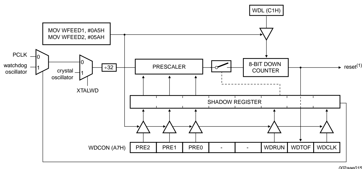
Fig 14. Watchdog timer in Watchdog mode (WDTE = 1)
