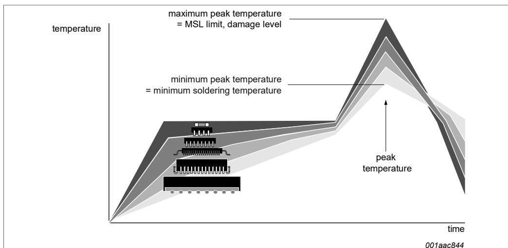
Figure 26. Temperature profiles for large and small components
