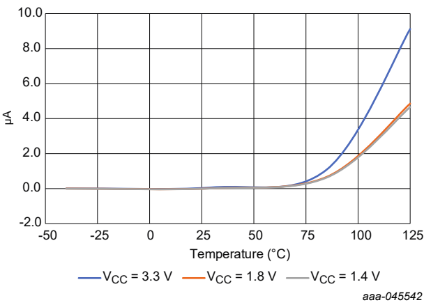
Figure 24. Shutdown current versus temperature
