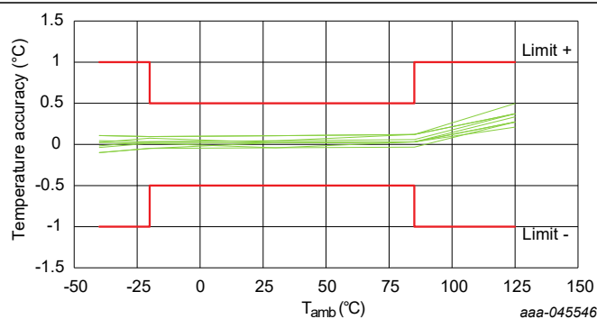
Figure 28. Accuracy vs temperature ( V_{CC} = 1.4\text{ V} to 3.6\text{ V} )
