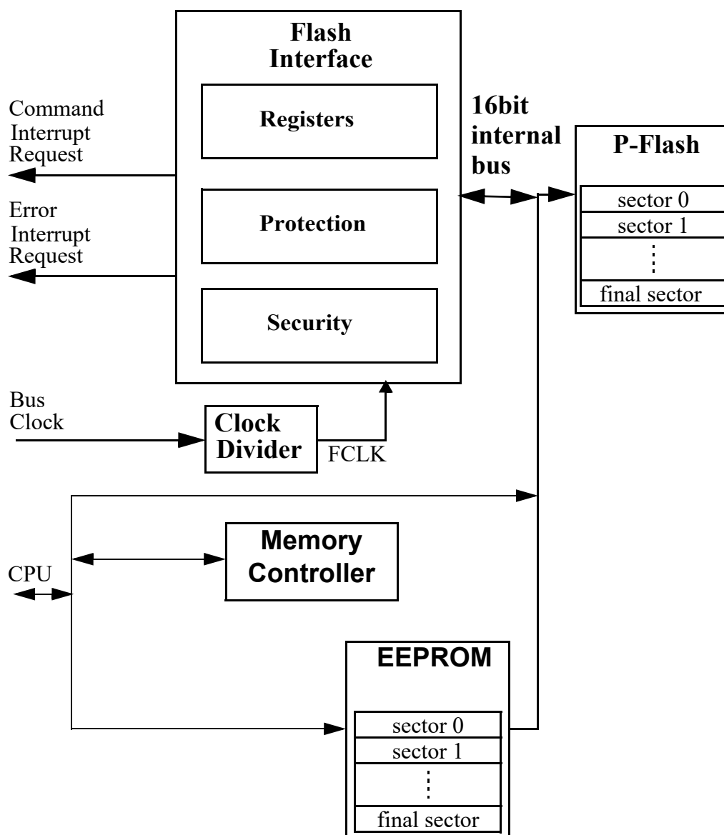
Figure 22-1. FTMZ Block Diagram
