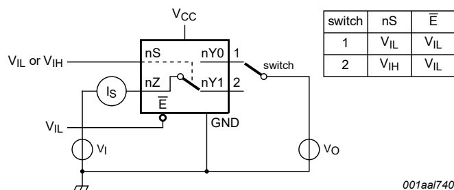
Figure 6. Test circuit for measuring ON-state leakage current
