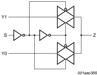
Fig 2. Logic diagram
