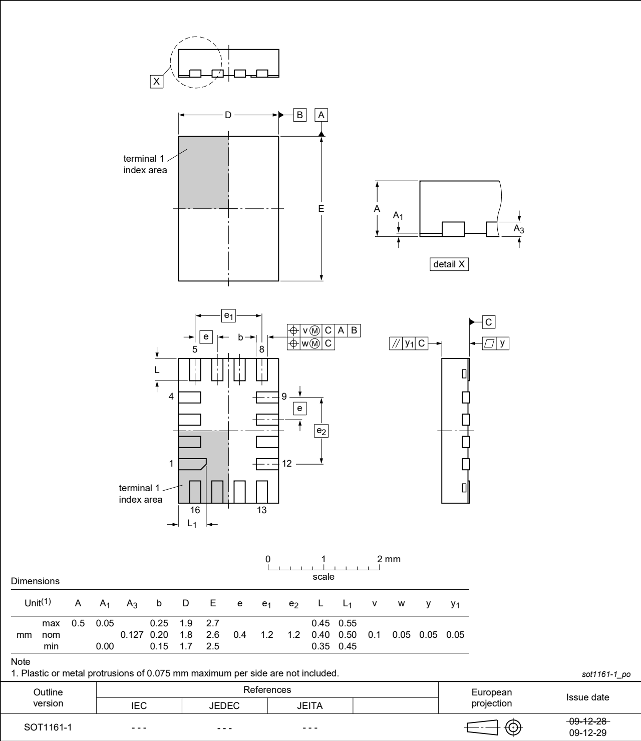
Figure 25. Package outline SOT1161-1 (XQFN16)
