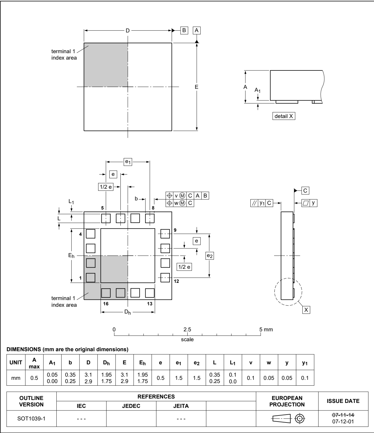
Figure 24. Package outline SOT1039-1 (HXQFN16U)
