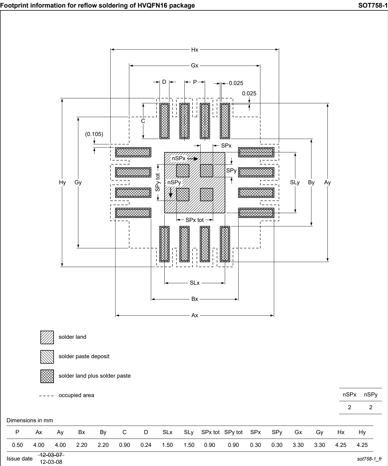
Figure 23. PCB footprint for SOT758-1 (HVQFN16); reflow soldering
