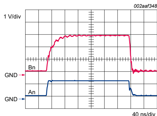
Figure 13. Example of typical AC waveform
