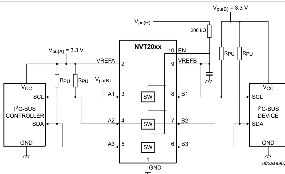
Figure 9. Bidirectional level shifting between two different power domains
