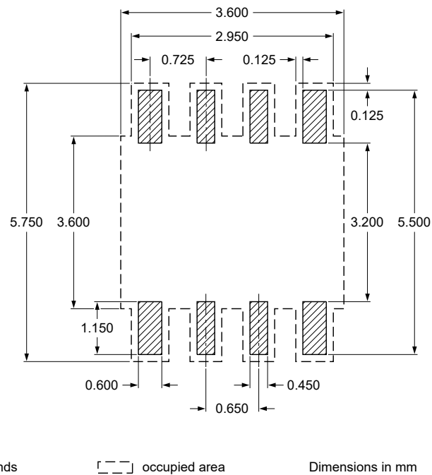
Figure 22. PCB footprint for SOT505-1 (TSSOP8); reflow soldering
