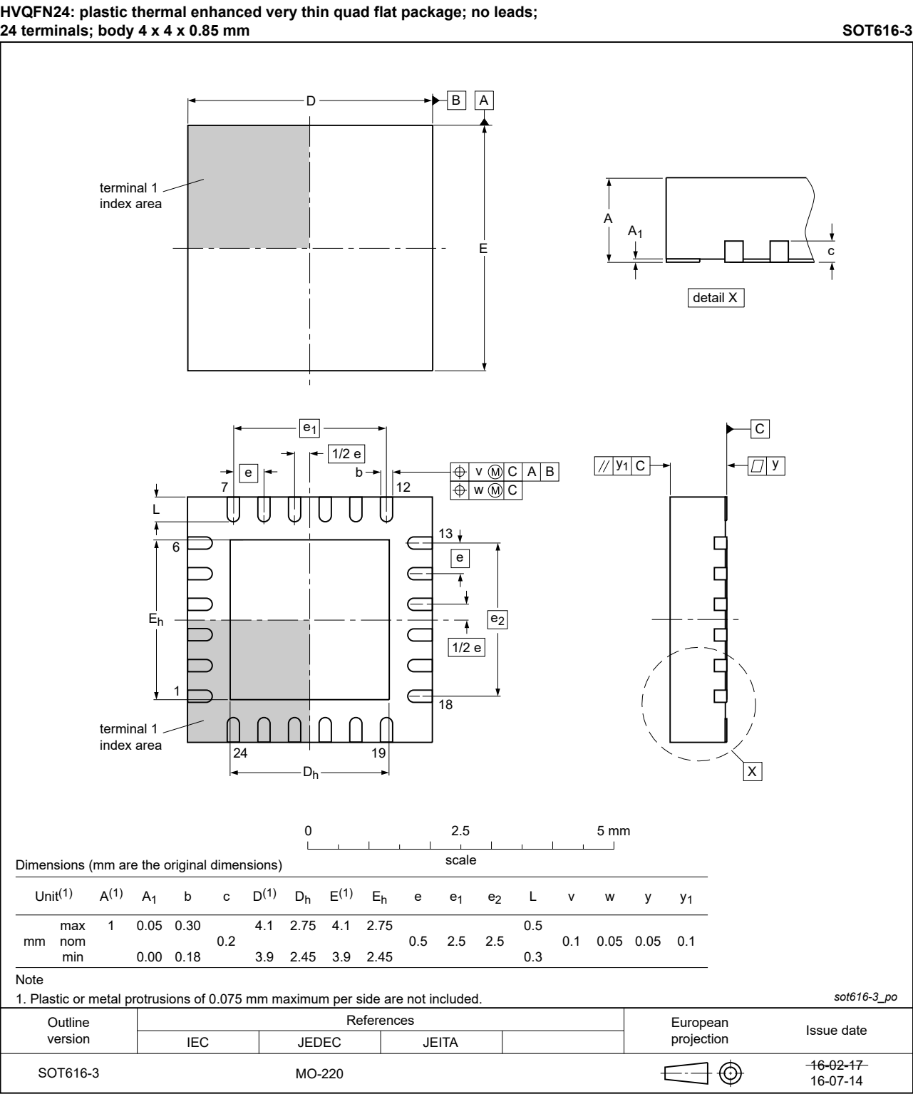
Figure 16. Package outline
