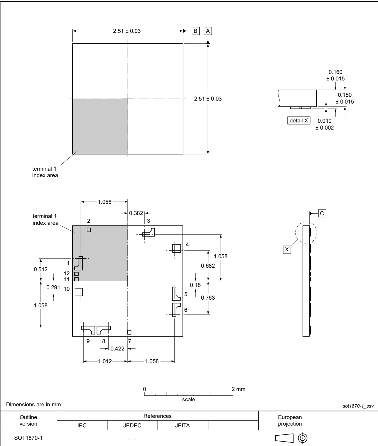
Bumped die with 8 functional bumps; 2.51 mm x 2.51 mm x 0.16 mm
