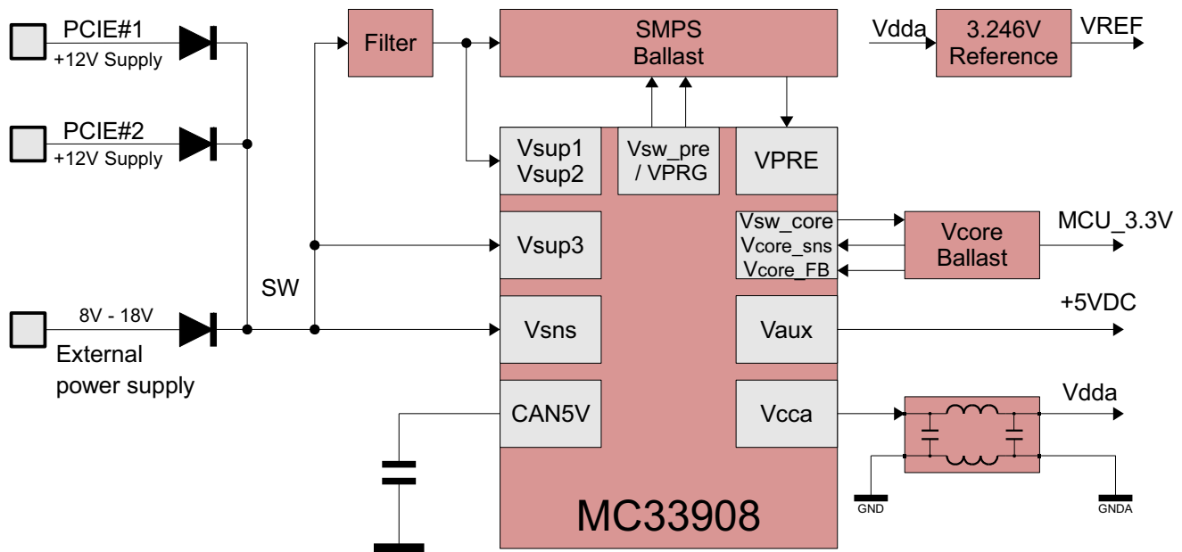
Figure 3-3. Power supply
