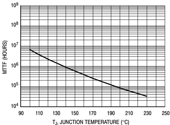
This above graph displays calculated MTTF in hours when the device is operated at V_{DD} = 28 Vdc, P_{out} = 35.5 W CW, and \eta_D = 57\% . MTTF calculator available at http://www.freescale.com/rf . Select Software & Tools/Development Tools/Calculators to access MTTF calculators by product.
