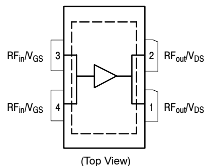
Figure 1. Pin Connections
