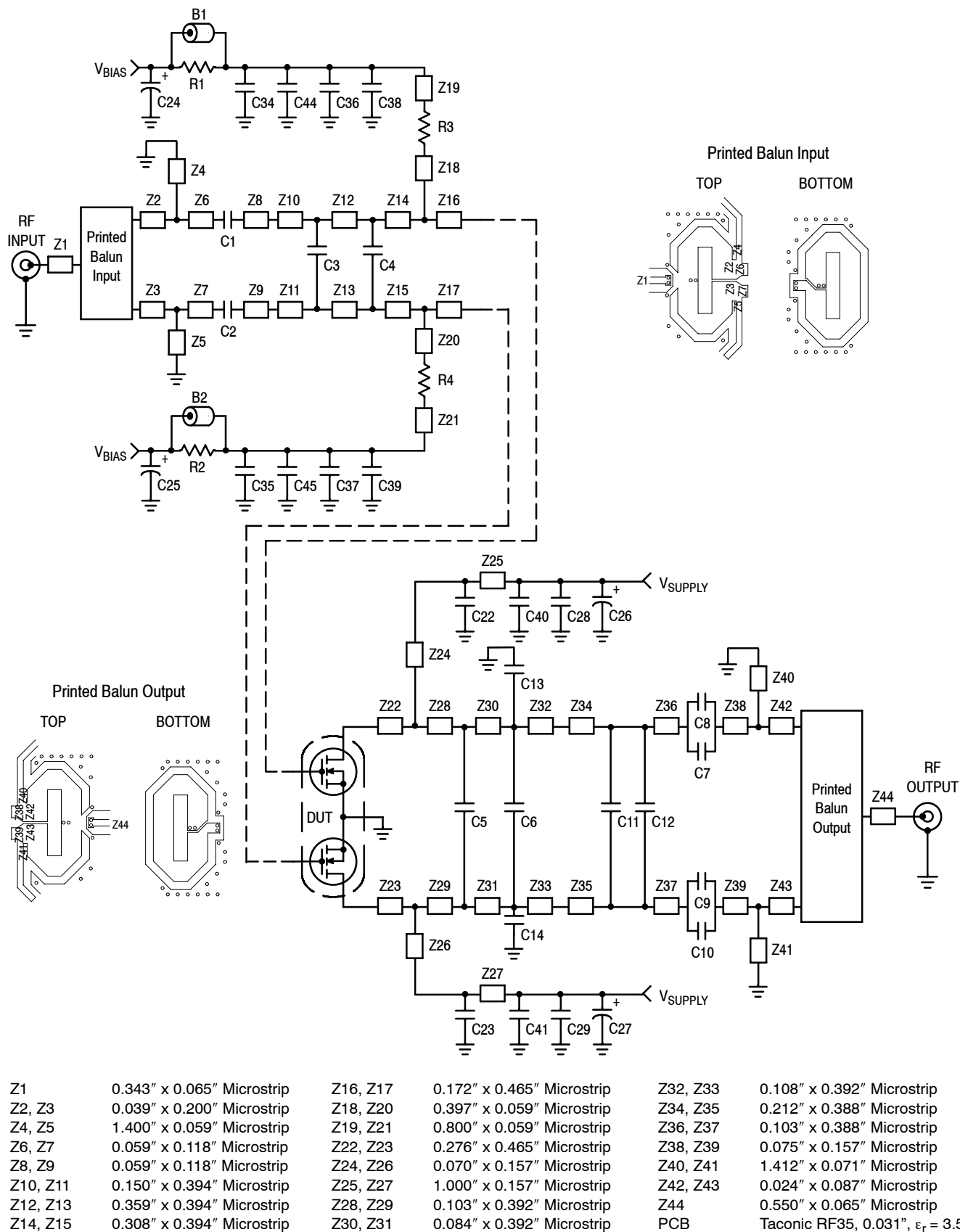
Figure 2. MRF6VP3450HR6(HSR6) Test Circuit Schematic
