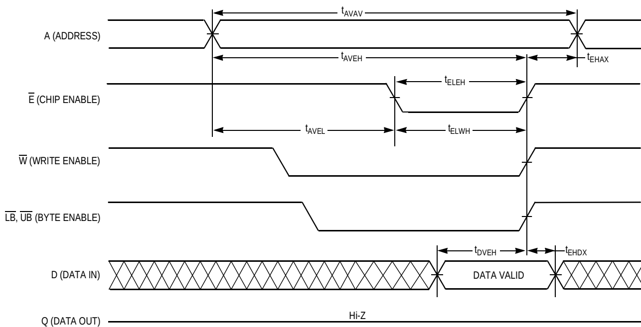
Figure 7. Write Cycle 2 ( \overline{E} Controlled)
