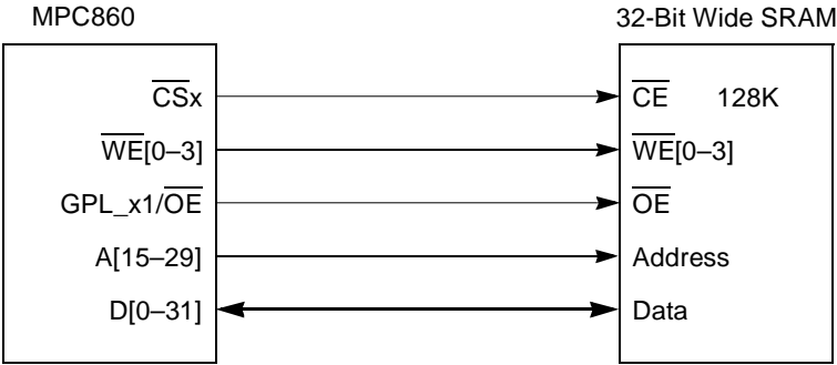
Figure 15-15. GPCM-to-SRAM Configuration
