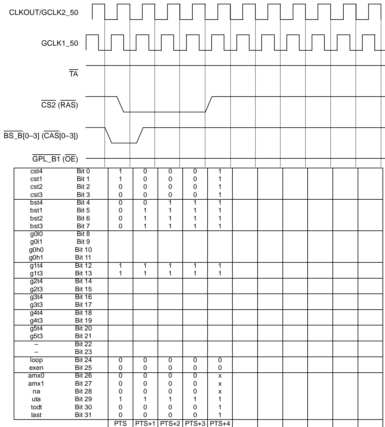
Figure 15-68. EDO DRAM Refresh Cycle ( \overline{\text{CAS}} Before \overline{\text{RAS}} )
