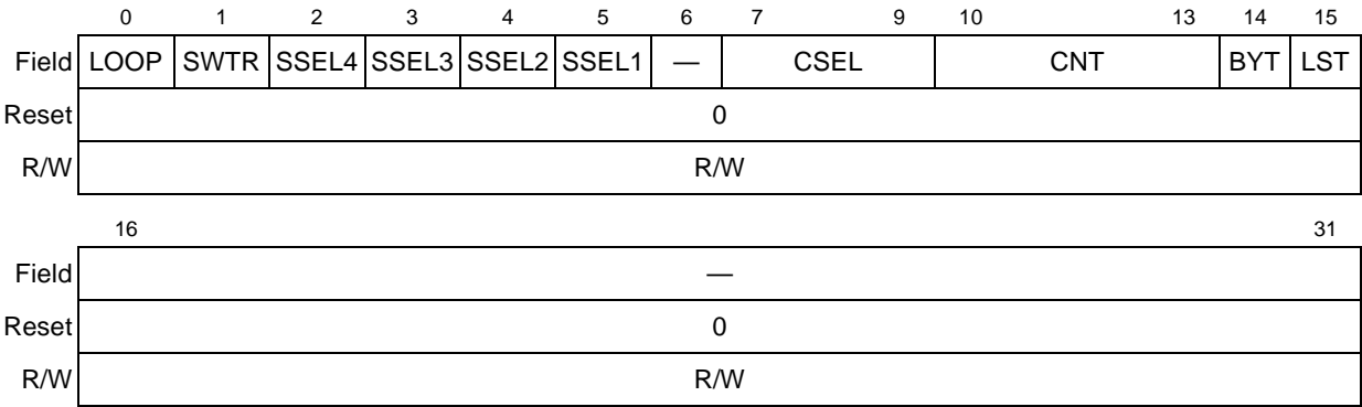
Figure 20-10. S1RAM Entry
