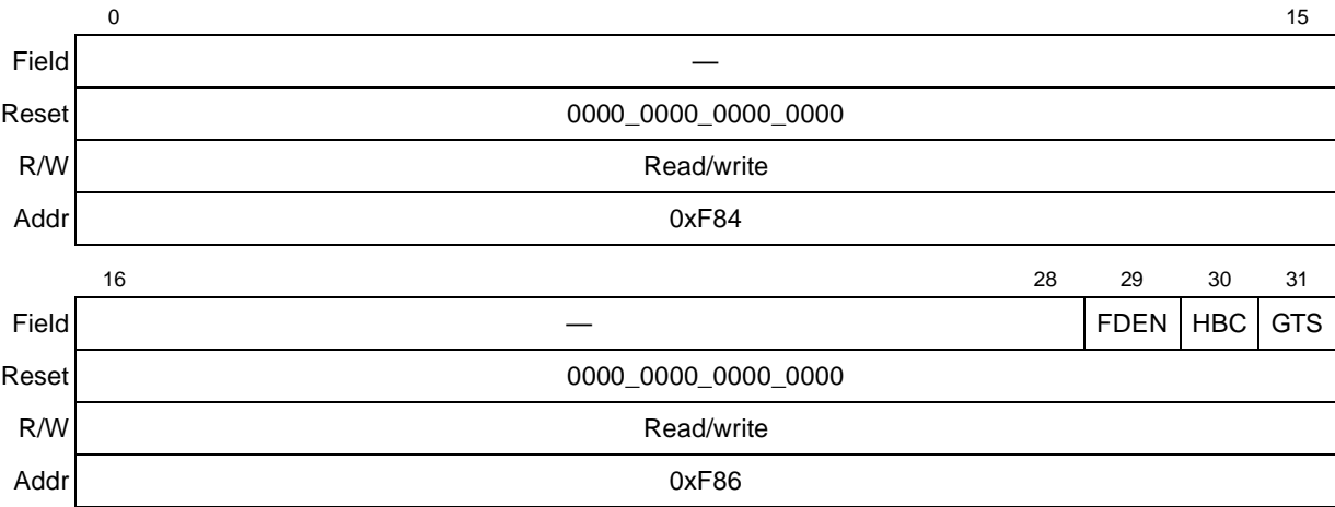
Figure 43-25. X_CNTRL Register
