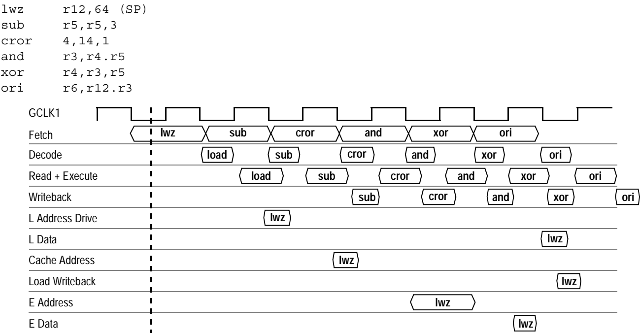
Figure 9-4. Private Writeback Bus Load Timing
