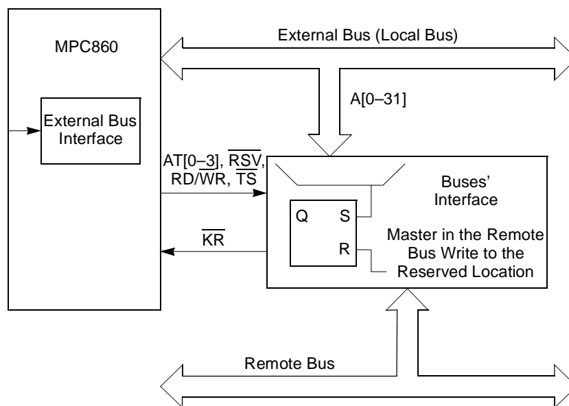
Figure 13-28. Reservation on Multilevel Bus Hierarchy
