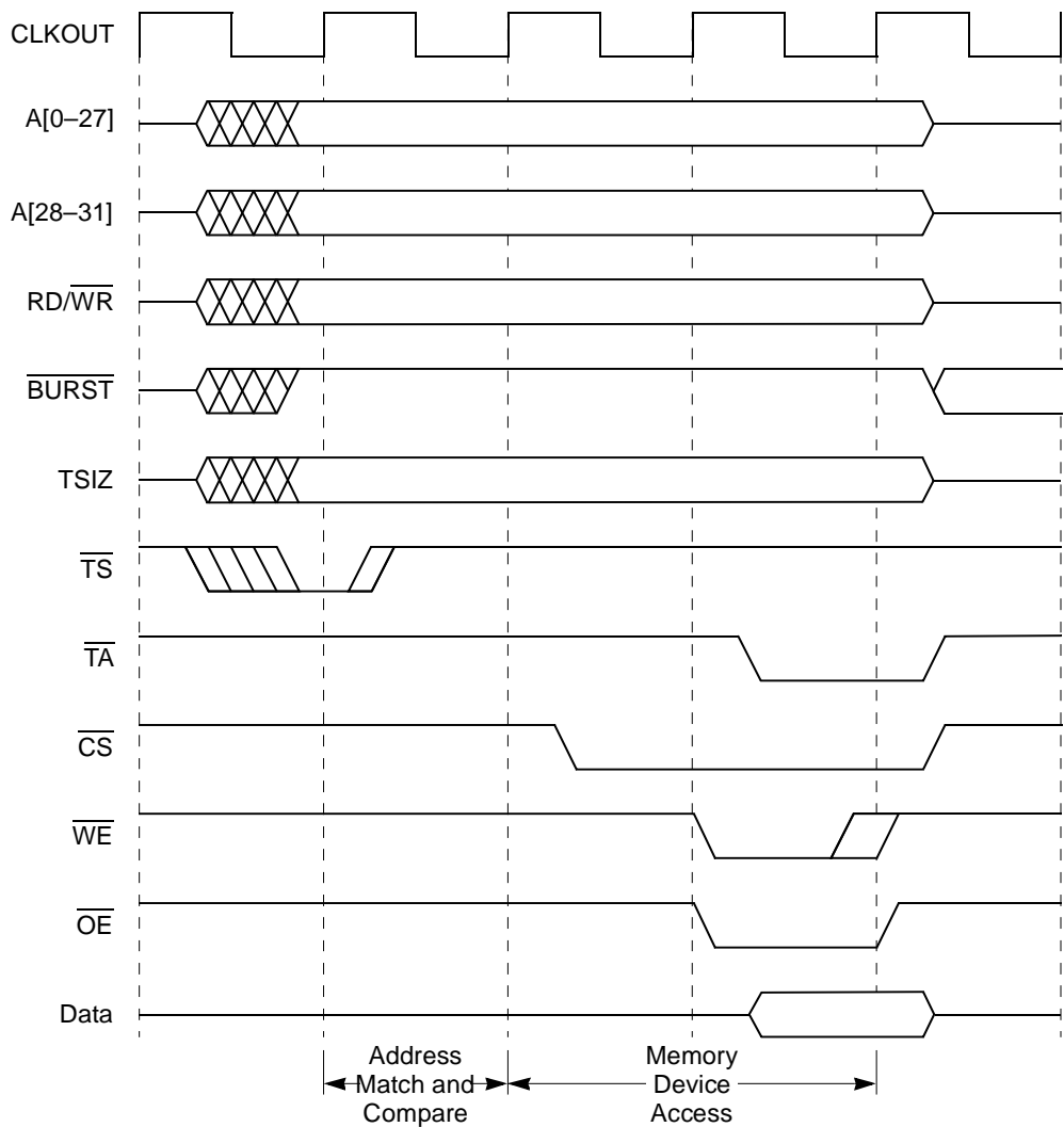
Figure 15-47. Synchronous External Master Access
