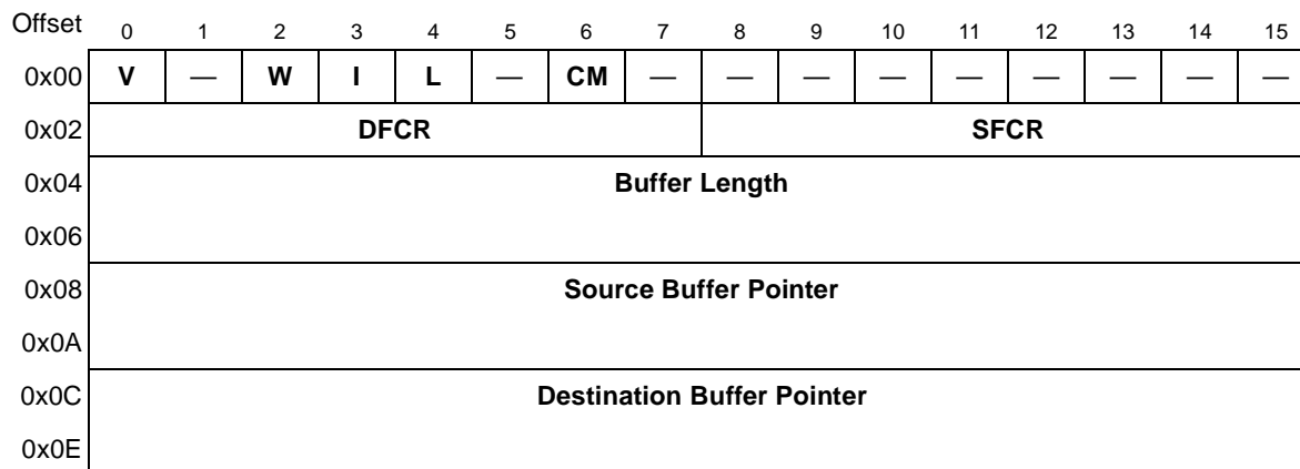
Figure 19-8. IDMA Buffer Descriptor Structure
