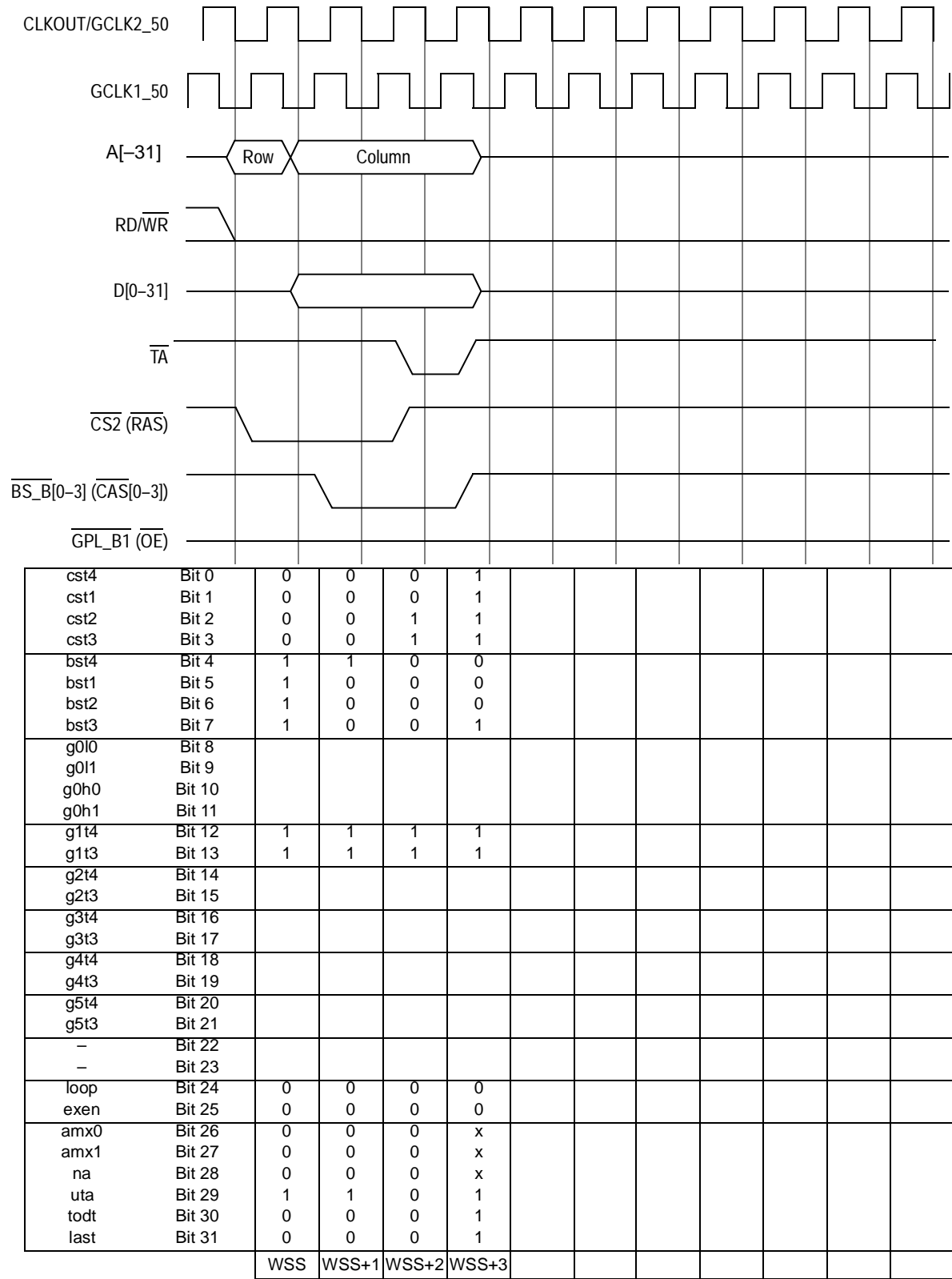
Figure 15-65. EDO DRAM Single-Beat Write Access
