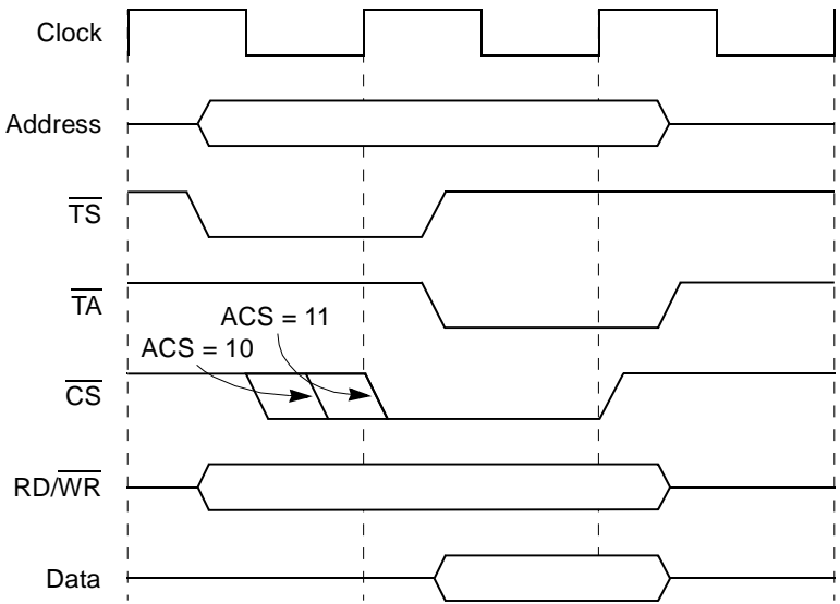
Figure 15-17. GPCM Peripheral Device Basic Timing (ACS = 1x and TRLX = 0)
