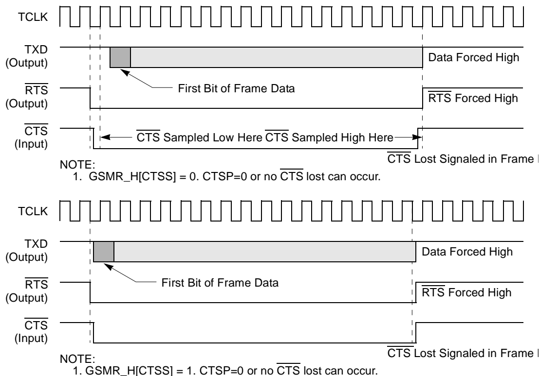
Figure 21-11. CTS Lost in Synchronous Protocols
