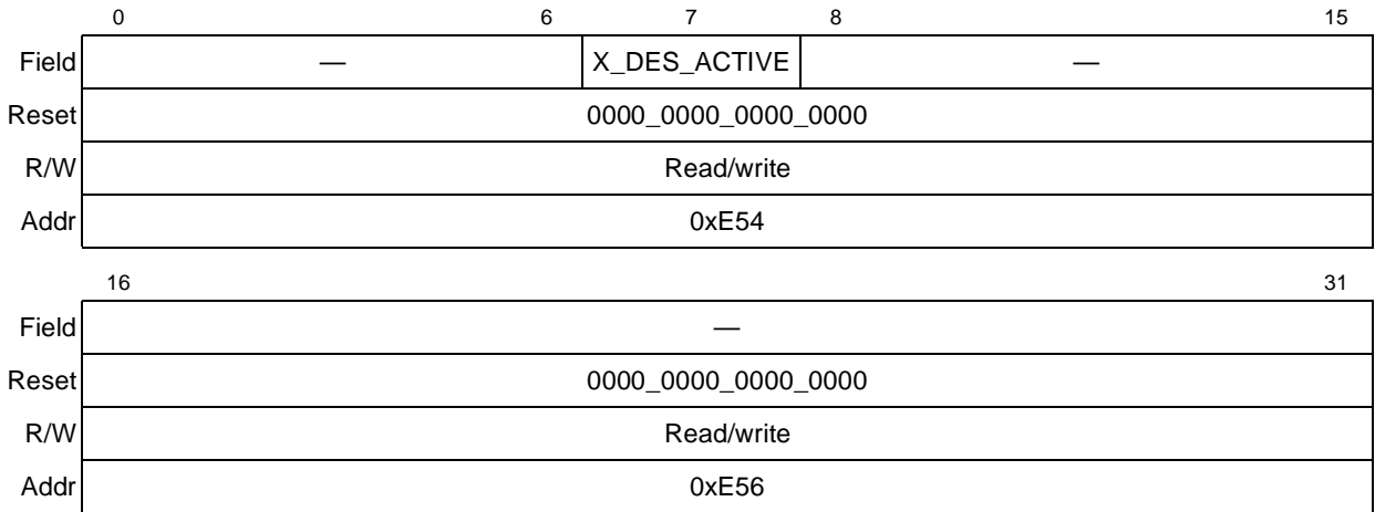
Figure 43-15. X_DES_ACTIVE Register
