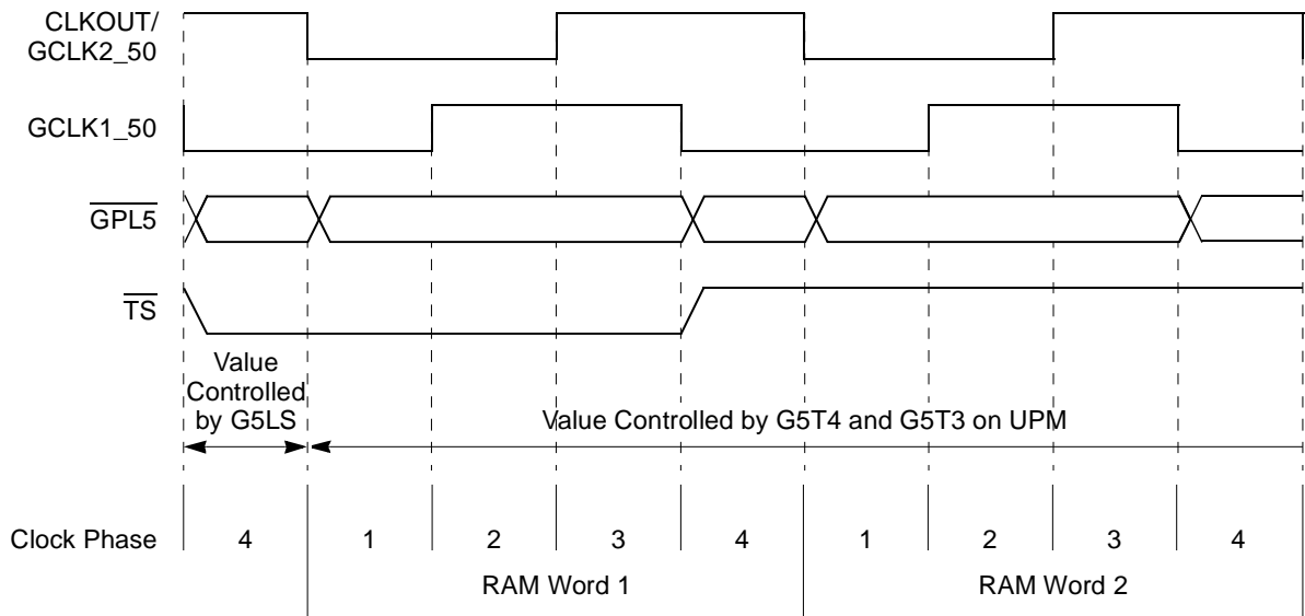
Figure 15-42. Early \overline{GPL5} Control
