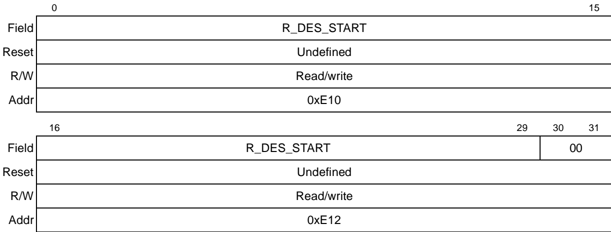
Figure 43-8. R_DES_START Register
