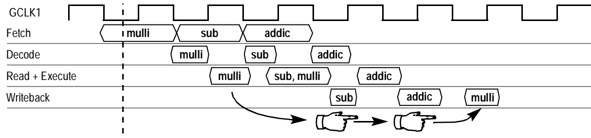
Figure 9-3. Writeback Arbitration Timing—Example 2
