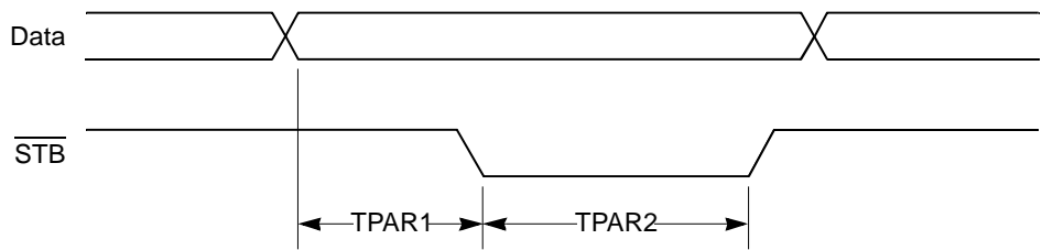
Figure 32-14. PIP Transmitter Timing Diagram
