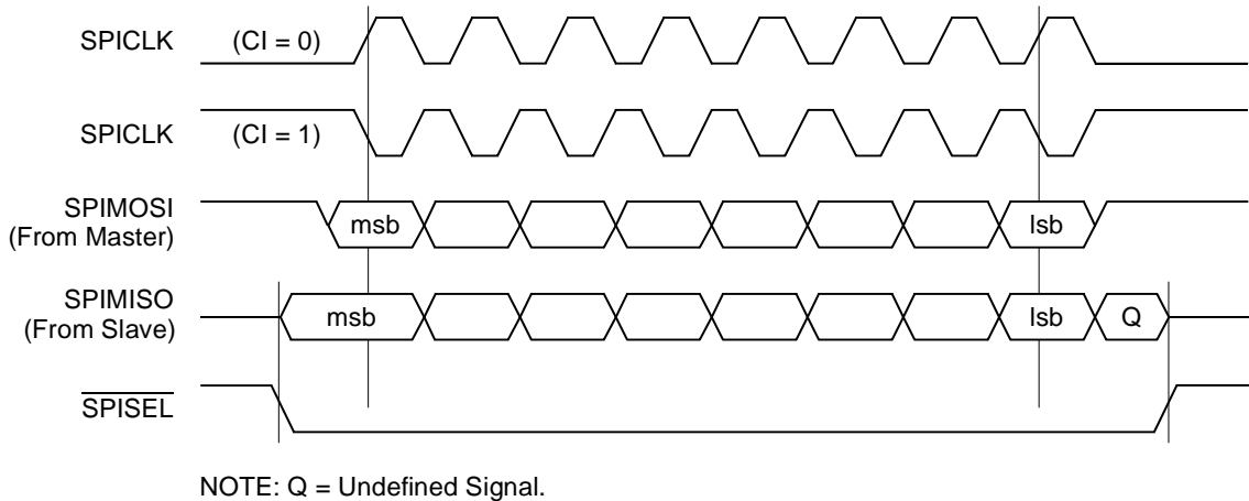
Figure 30-5. SPI Transfer Format with SPMODE[CP] = 0
