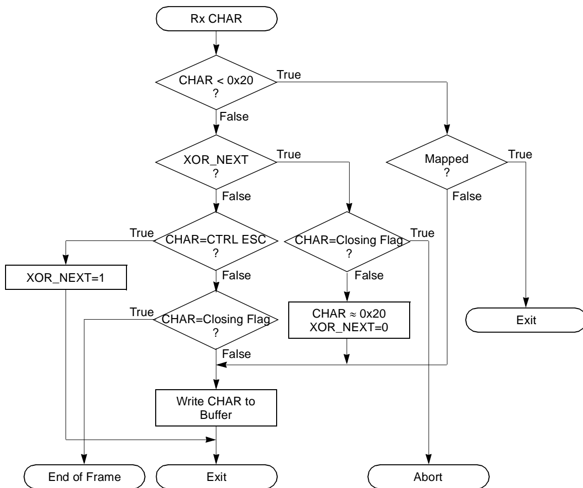
Figure 25-2. Receive Flowchart
