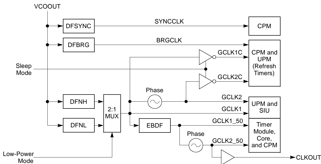
Figure 14-5. Clock Dividers
