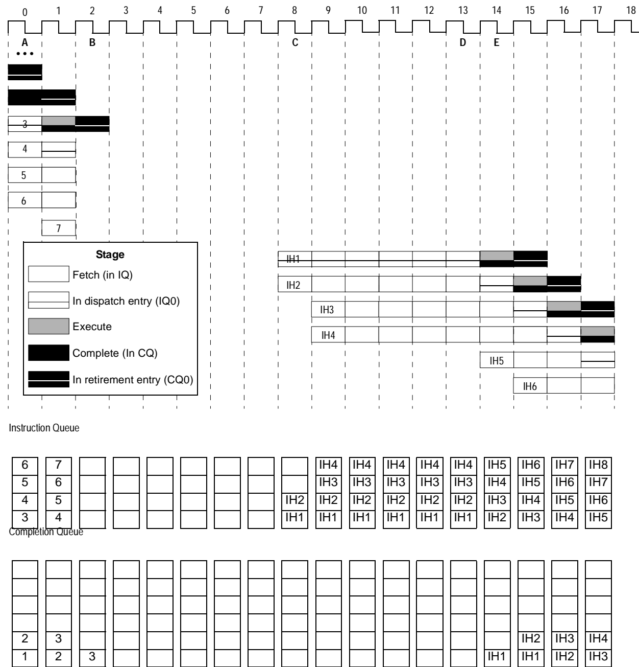
Figure 6-1. Exception Latency
