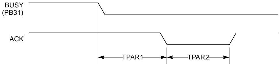
Figure 32-15. PIP Receiver Timing—Mode 0
