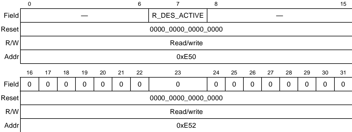
Figure 43-14. R_DES_ACTIVE Register
