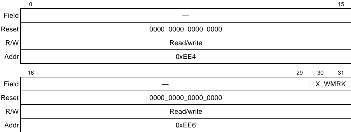
Figure 43-20. X_WMRK Register
