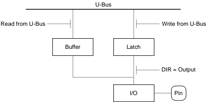
Figure 32-8. Port B General-Purpose I/O
