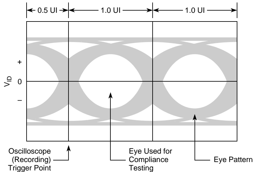
Figure 41. Example Receiver Input Eye Pattern
