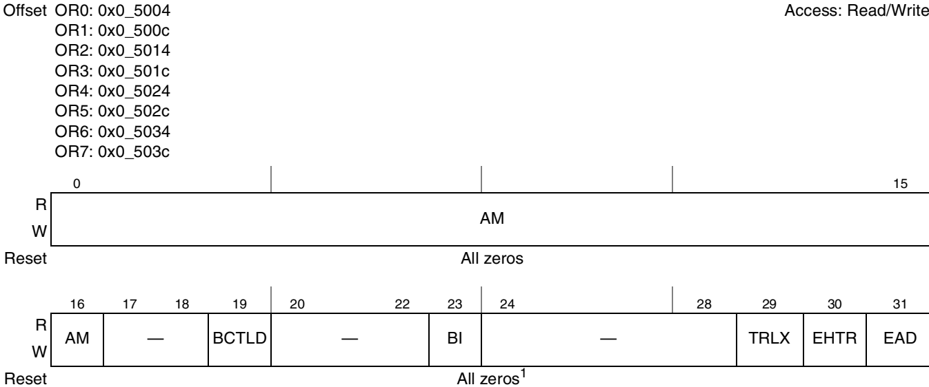
Figure 10-5. Option Registers (OR n ) in UPM Mode
