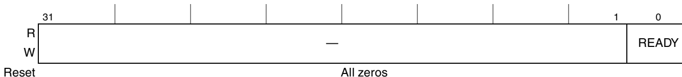
Figure 15-112. PCI Express Inbound Mailbox Control Register (PEX_IMBCR)
