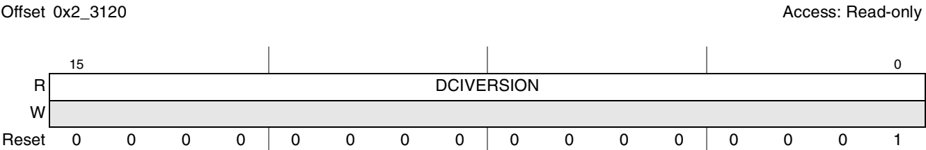
Figure 20-6. Device Interface Version (DCIVERSION)
