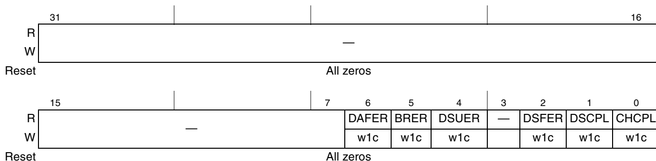
Figure 15-106. PCI Express Write DMA Status Register (PEX_WDMA_STAT)
