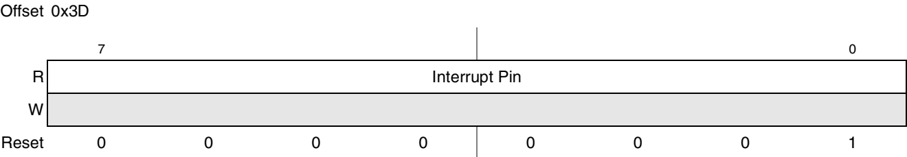
Figure 14-39. Interrupt Pin Register
