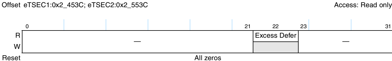
Figure 18-46. Interface Status Register Definition
