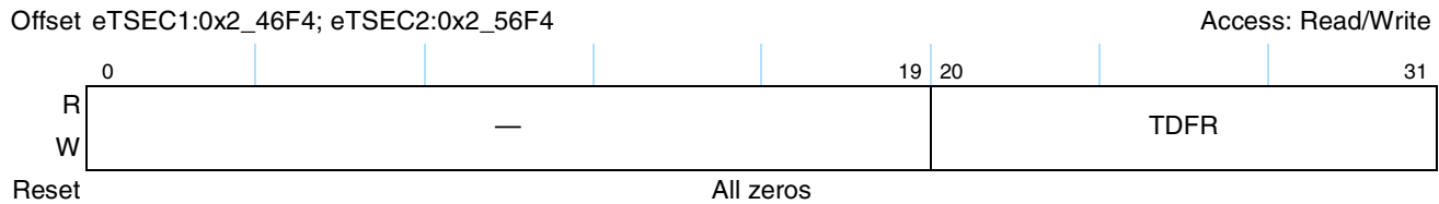
Figure 18-80. Transmit Deferral Packet Counter Register Definition
