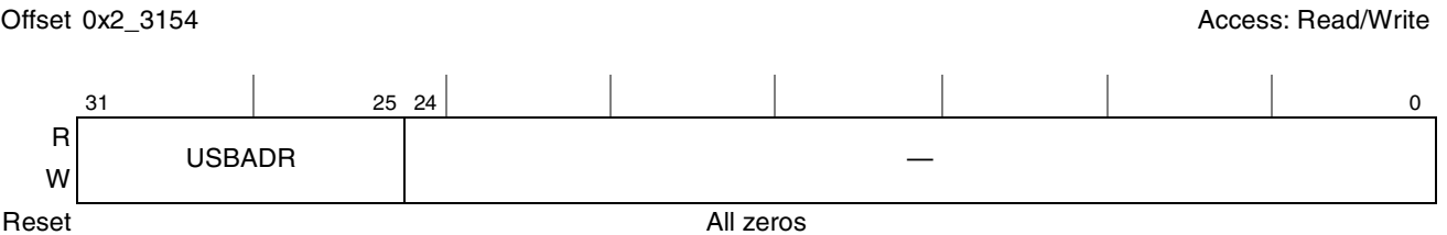
Figure 20-13. Device Address (DEVICEADDR)
