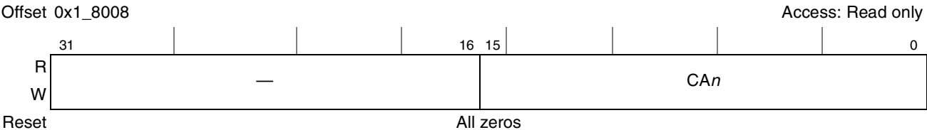
Figure 16-3. Command Active Register (CAR)
