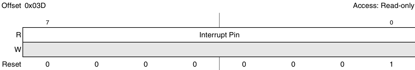
Figure 15-20. PCI Express Interrupt Pin Register
