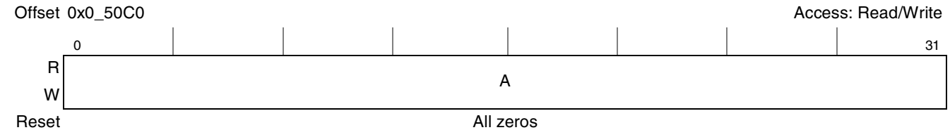
Figure 10-17. Transfer Error Address Register (LTEAR)
