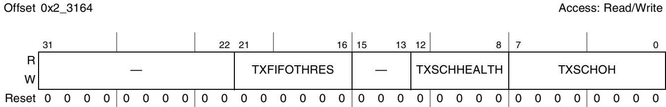
Figure 20-17. Transmit FIFO Tuning Controls (TXFILLTUNING)
