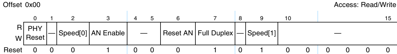
Figure 18-114. Control Register Definition
