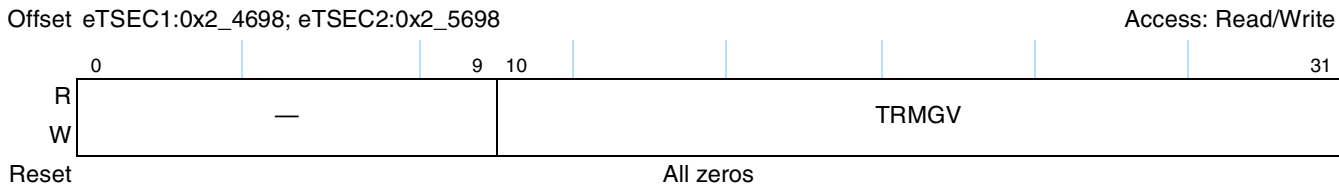
Figure 18-57. Transmit and Received 1519- to 1522-Byte VLAN Frame Register Definition
