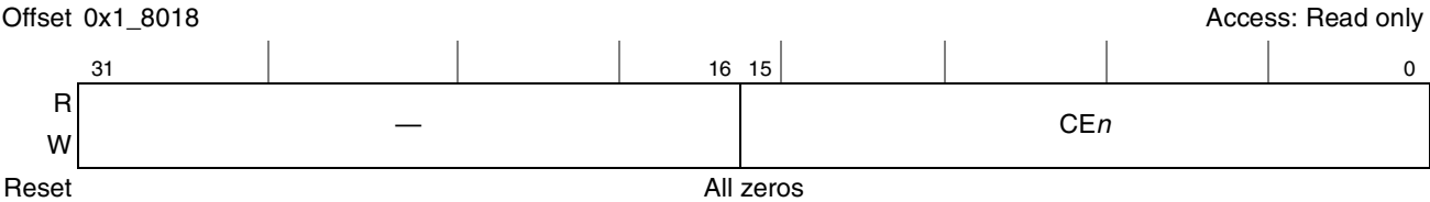
Figure 16-5. Command Error Register (CER)
