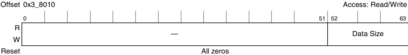
Figure 17-34. AFEU Context/Data Size Register
