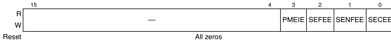
Figure 15-60. PCI Express Root Control Register
