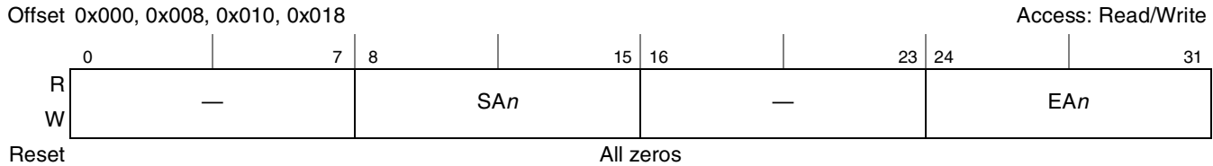
Figure 9-2. Chip Select Bounds Registers ( CS_n\_BNDS )
