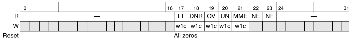
Figure 23-7. SPIE—SPI Event Register Definition
