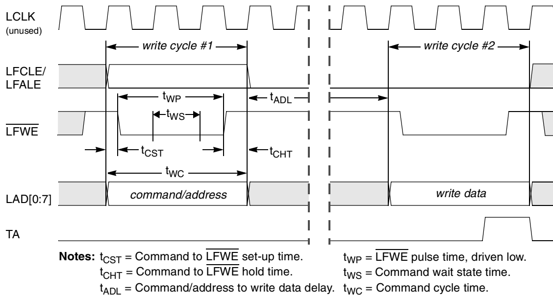
Figure 10-52. Timing of FCM Command/Address and Write Data Cycles (for TRLX = 0 , CHT = 0 , CST = 1 , SCY = 1 , CLKDIV = 4 \cdot N )
