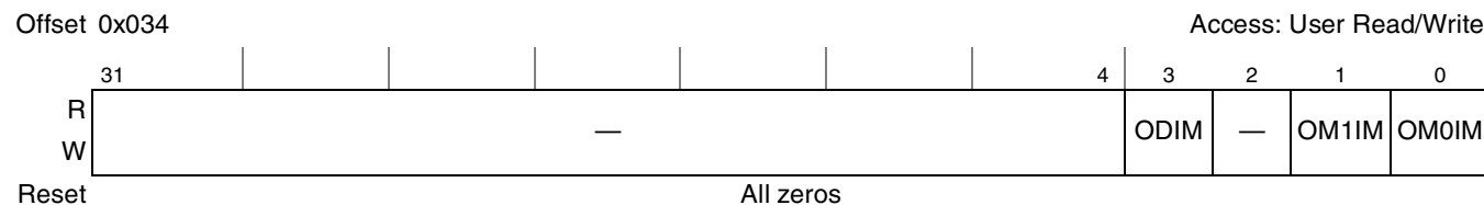
Figure 13-3. Outbound Message Interrupt Mask Register (OMIMR)
