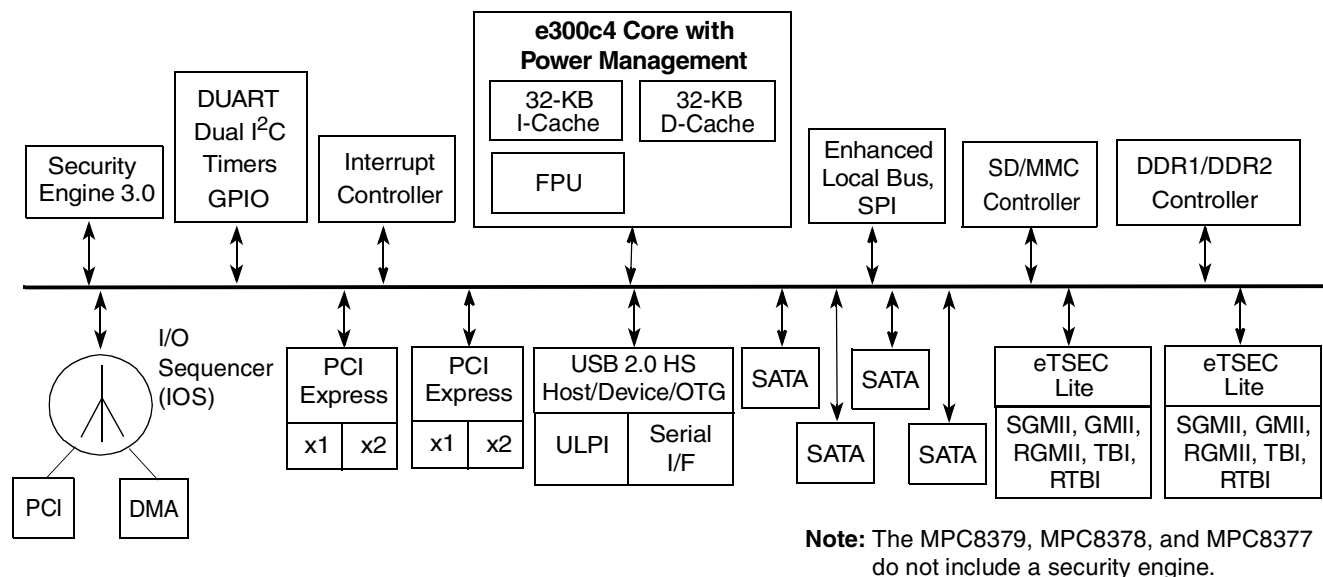
Figure 1-1. MPC8379E Block Diagram
