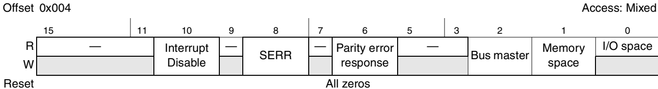
Figure 15-5. PCI Express Command Register
