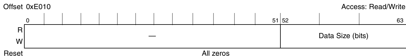
Figure 17-64. KEU Data Size Register
