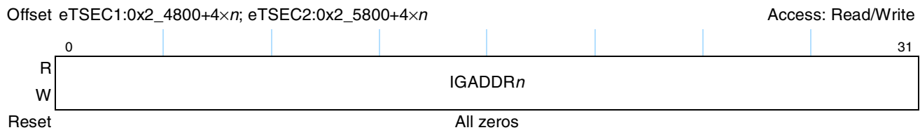
Figure 18-99. IGADDR n Register Definition
