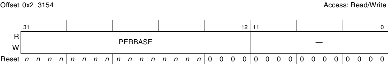
Figure 20-12. Periodic Frame List Base Address (PERIODICLISTBASE)
