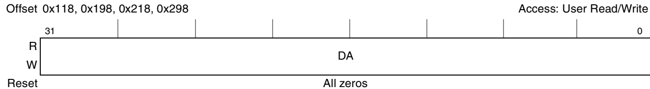
Figure 13-14. DMA Destination Address Register (DMADAR n )
