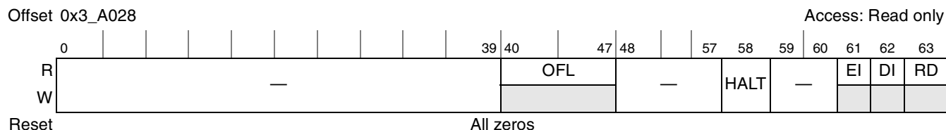
Figure 17-104. RNGU Status Register
