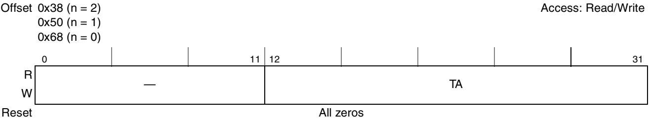
Figure 14-15. PCI Inbound Translation Address Registers (PITAR n )
