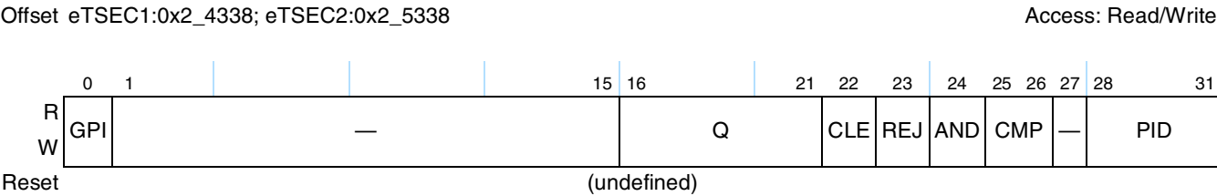
Figure 18-28. Receive Queue Filer Table Control Register Definition
