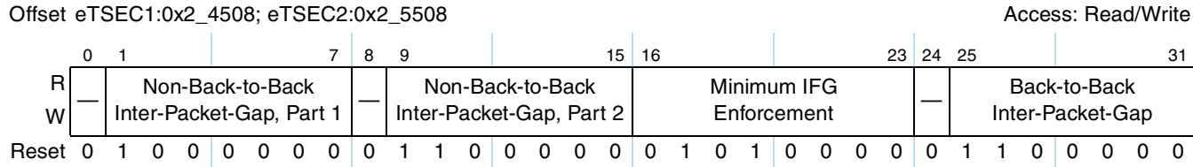
Figure 18-37. IPGIFG Register Definition
