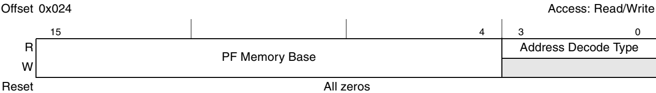
Figure 15-32. PCI Express Prefetchable Memory Base Register
