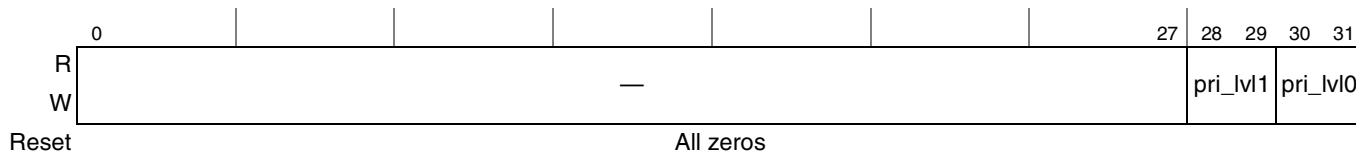
Figure 20-32. Priority Control (PRI CTRL)
