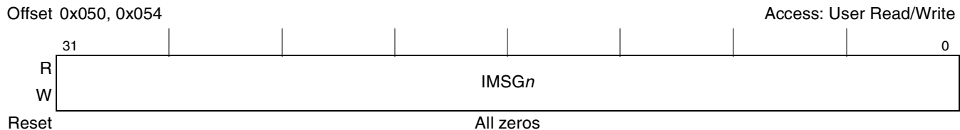
Figure 13-4. Inbound Message Registers (IMR0, IMR1)
