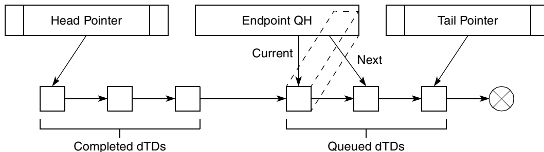
Figure 20-65. Software Link Pointers
