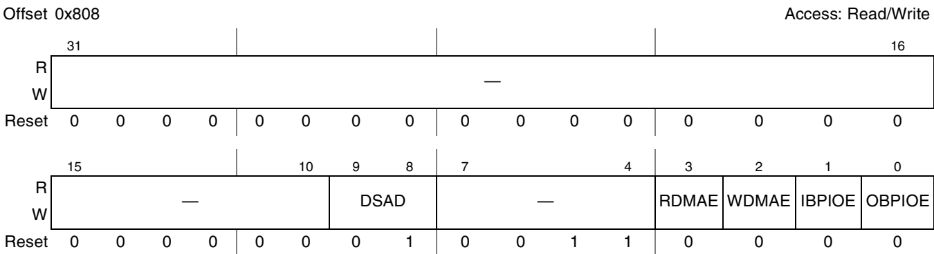
Figure 15-97. PCI Express CSB Bridge Control Register (PEX_CSB_CTRL)
