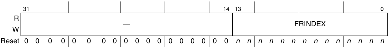
Figure 20-11. USB Frame Index (FRINDEX)
