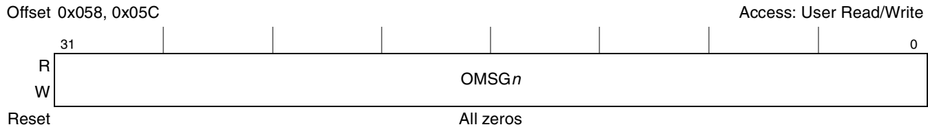
Figure 13-5. Outbound Message Registers (OMR0–OMR1)
