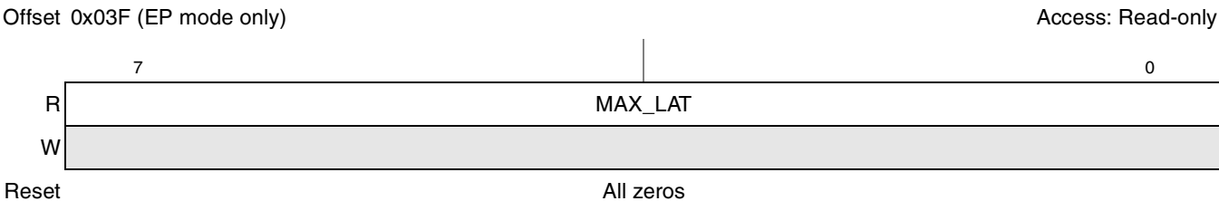
Figure 15-22. PCI Express Maximum Latency Register (MAX_LAT)
