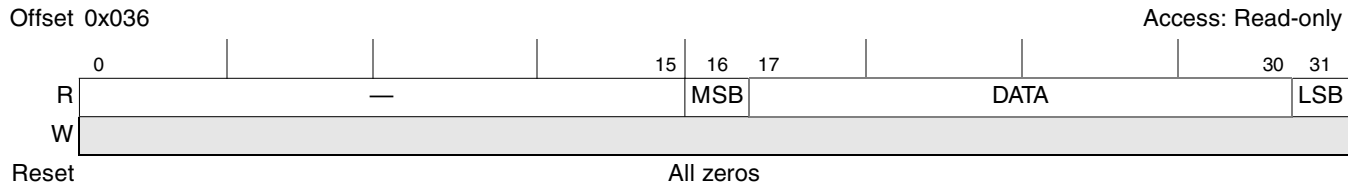
Figure 23-15. Example SPMODE[REV] = 0 SPMODE[LEN] = 15 LSB Sent First
