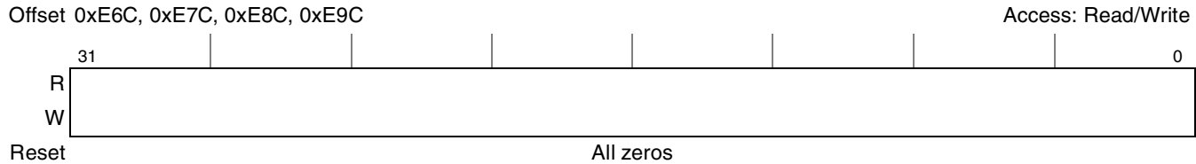
Figure 15-138. CI Express RC Inbound Window Base Address Register High n (PEX_RCIWBARH0–PEX_RCIWBARH3)
