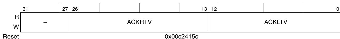
Figure 15-81. PCI Express ACK Replay Timeout Register
