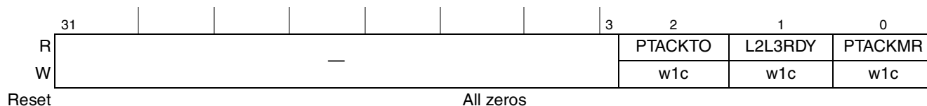
Figure 15-95. PME To Ack Status Register (PEX PME TO ACK SR)
