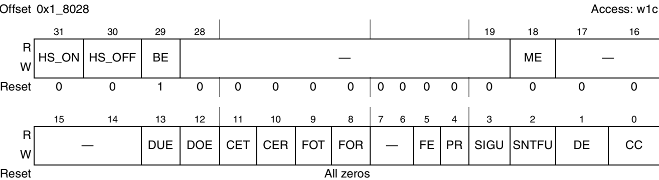
Figure 16-8. Host Status Register (HStatus)
