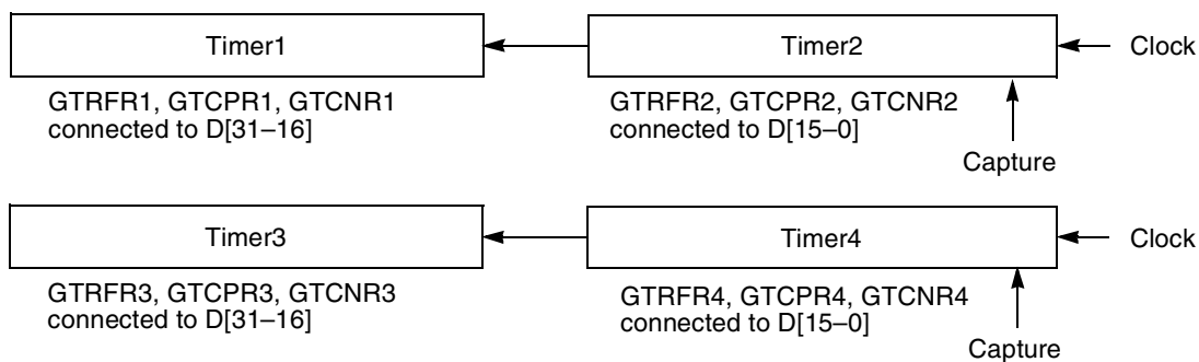
Figure 5-55. Timer Pair-Cascaded Mode Block Diagram
