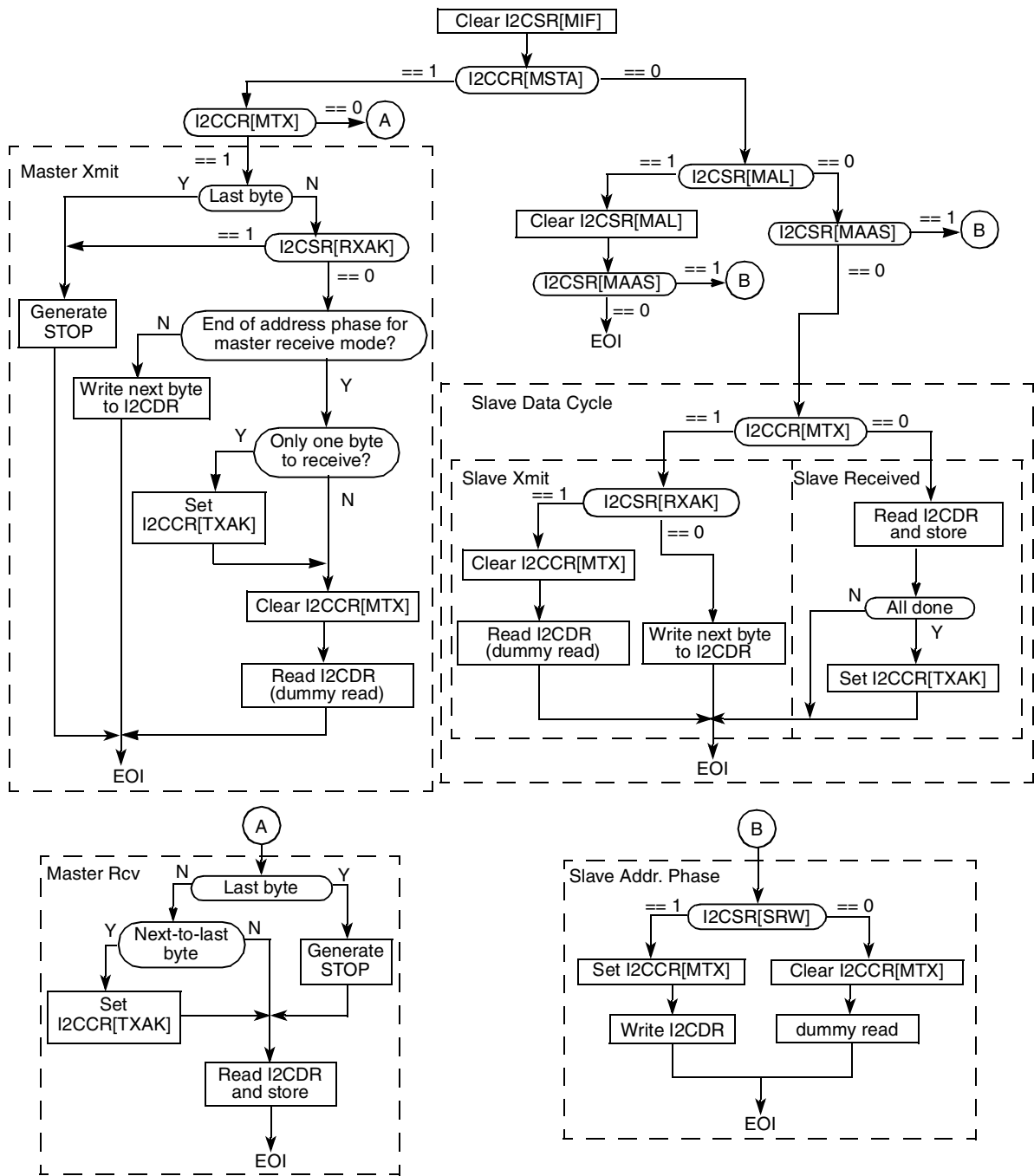
Figure 21-11. Example I 2 C Interrupt Service Routine Flowchart
