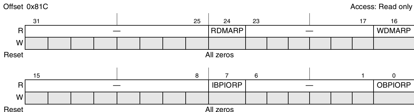
Figure 15-99. PCI Express CSB Bridge Status Register (PEX_CSB_STAT)
