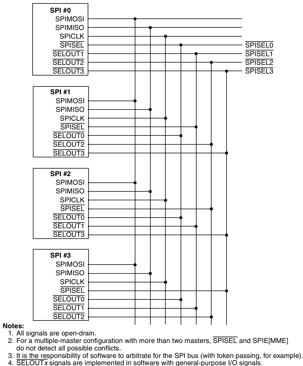
Figure 23-3. Multiple-Master Configuration
