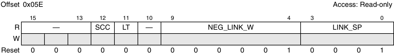
Figure 15-56. PCI Express Link Status Register
