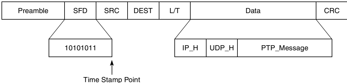
Figure 18-138. PTP Packet Format
