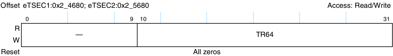
Figure 18-51. Transmit and Receive 64-Byte Frame Register Definition
