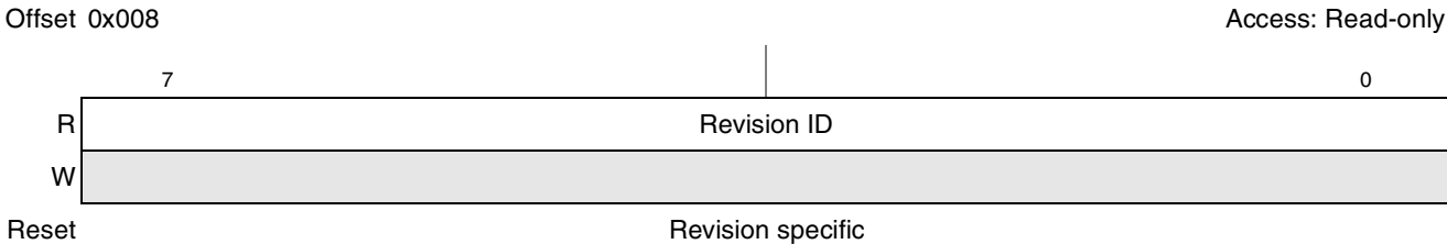
Figure 15-7. PCI Express Revision ID Register
