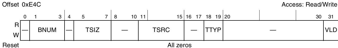
Figure 9-28. Memory Error Attributes Capture Register (CAPTURE_ATTRIBUTES)
