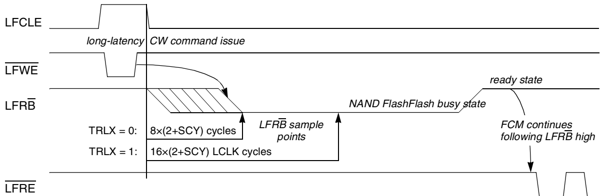
Figure 10-55. FCM Delay Prior to Sampling \text{LFR}\bar{\text{B}} State
