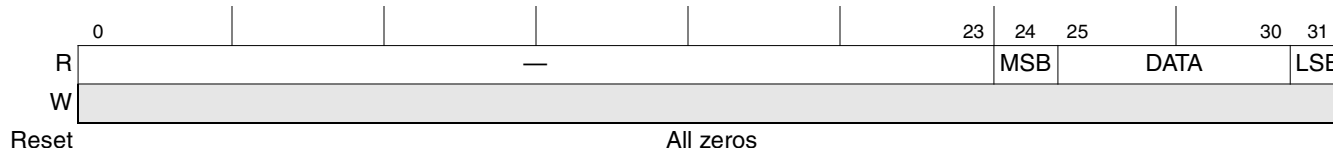
Figure 23-13. Example SPMODE[REV] = 1 SPMODE[LEN] = 7 MSB Sent First
