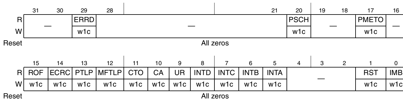
Figure 15-128. CSB System Miscellaneous Interrupt Status Register (PEX_CSMISR)
