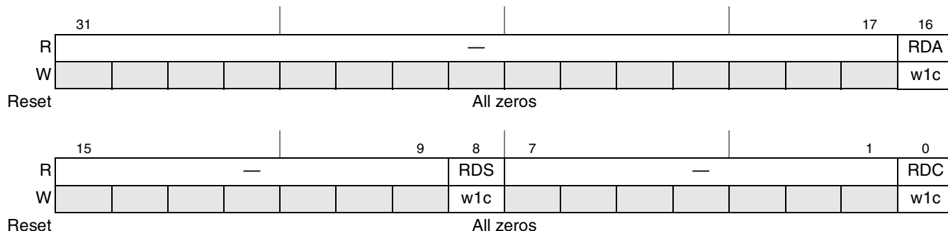
Figure 15-127. CSB System Read DMA Interrupt Status Register (PEX_CSRDISR)
