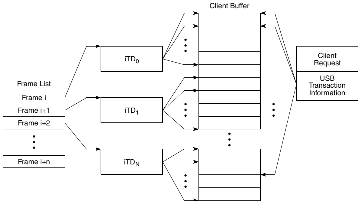
Figure 20-48. Example Association of iTDs to Client Request Buffer
