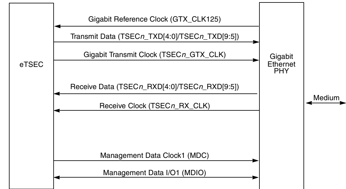
Figure 18-127. eTSEC-RTBI Connection
