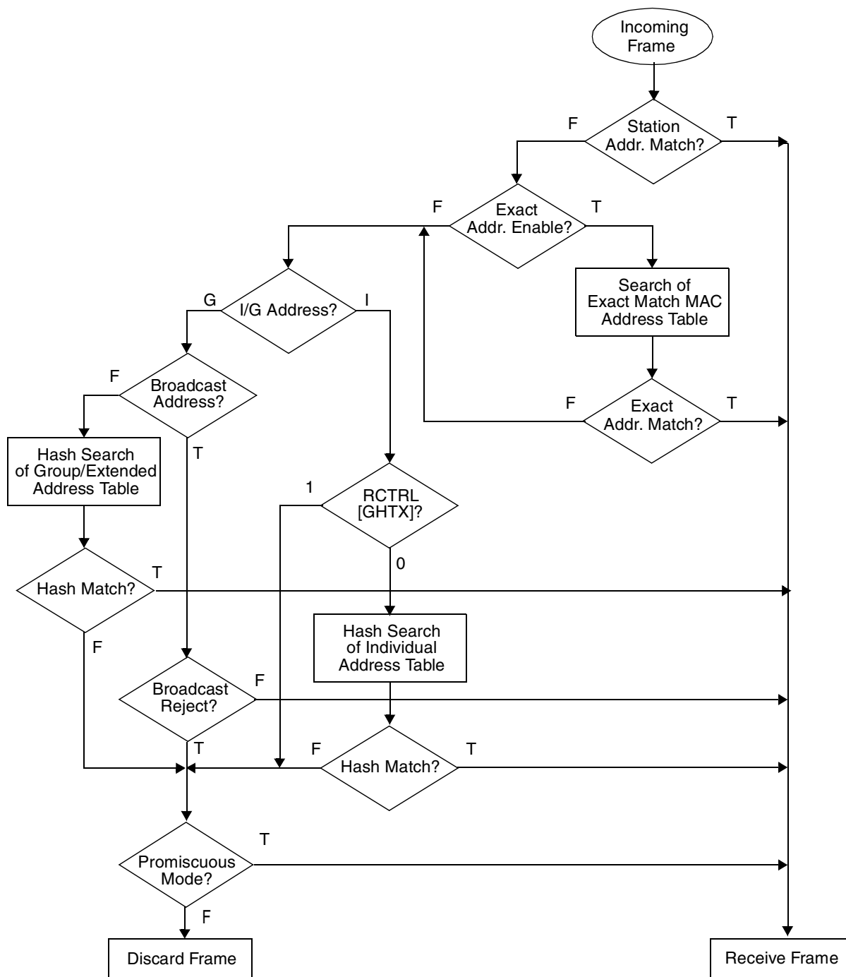
Figure 18-130. Ethernet Address Recognition Flowchart
