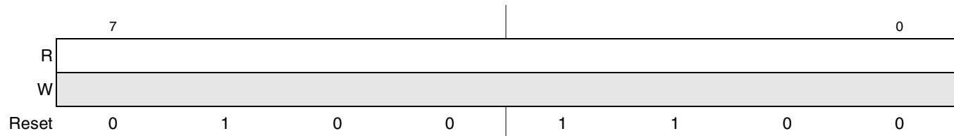
Figure 15-44. PCI Express Power Management Next Capabilities Pointer
