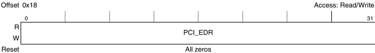
Figure 14-11. PCI Error Data Low Capture Register (PCI_EDLCR)
