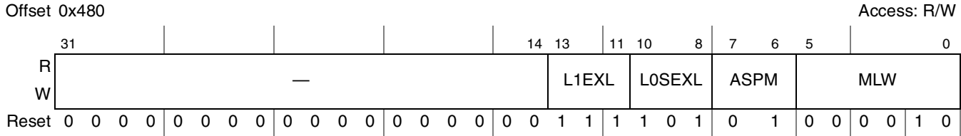
Figure 15-88. PCI Express Link Capabilities Update Register
