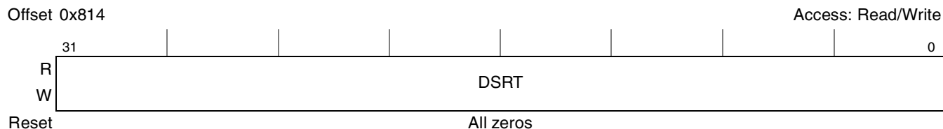
Figure 15-98. PCI Express DMA Descriptor Timer Register (PEX_DMA_DSTMR)
