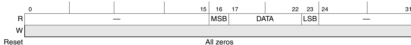
Figure 23-12. Example SPMODE[REV] = 0 SPMODE[LEN] = 7 LSB Sent First
