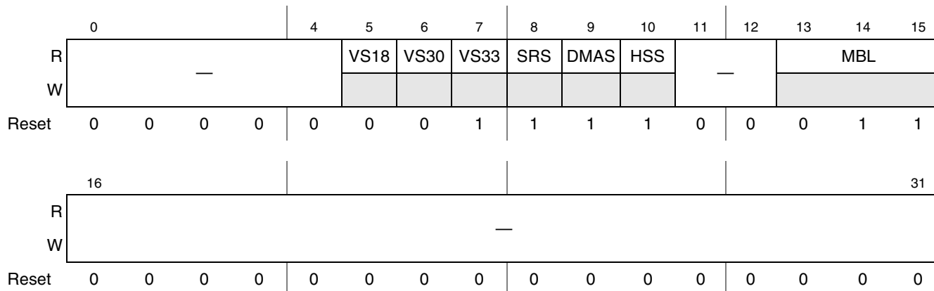
Figure 11-16. Host Capabilities Register (HOSTCAPBLT)
