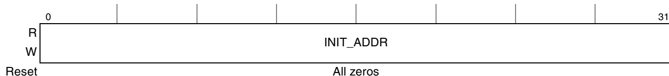
Figure 9-16. DDR Initialization Address Configuration Register (DDR_INIT_ADDR)
