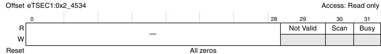
Figure 18-45. MII Mgmt Indicator Register Definition
