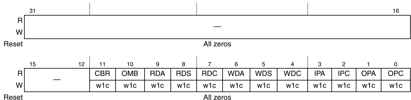
Figure 15-115. PCI Express Host Interrupt Status Register (PEX_HISR)
