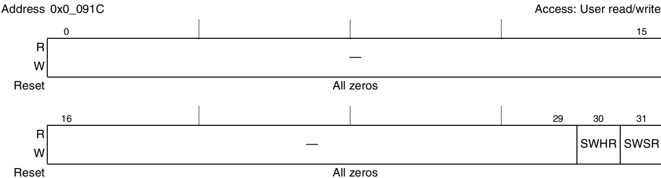
Figure 4-12. Reset Control Register (RCR)
