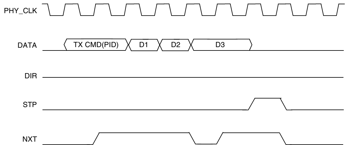
Figure 20-69. ULPI Data Transmit (PID)
