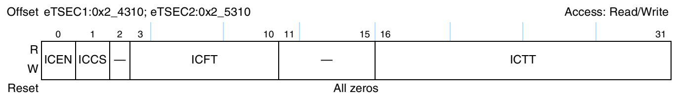
Figure 18-24. RXIC Register Definition
