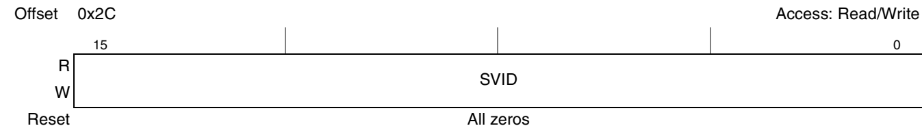
Figure 14-35. Subsystem Vendor ID Configuration Register
