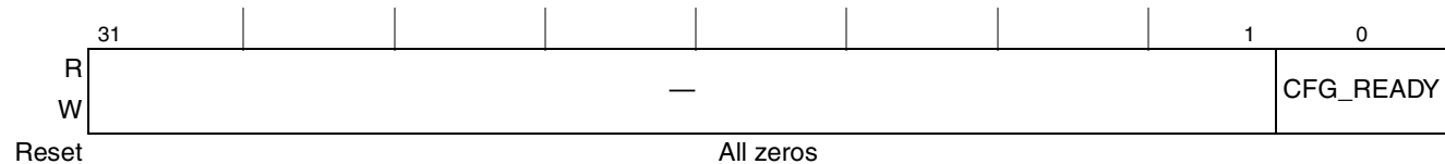
Figure 15-90. PCI Express Configuration Ready Register (PEX_CFG_READY)
