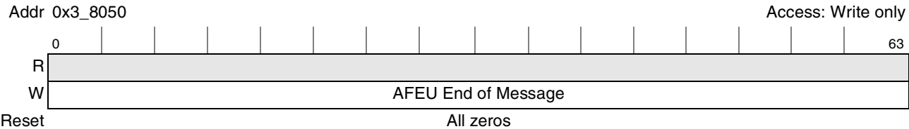
Figure 17-39. AFEU End of Message Register
