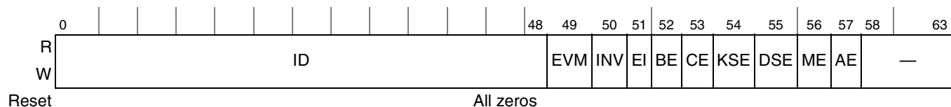
Figure 17-98. PKEU Interrupt Status Register
