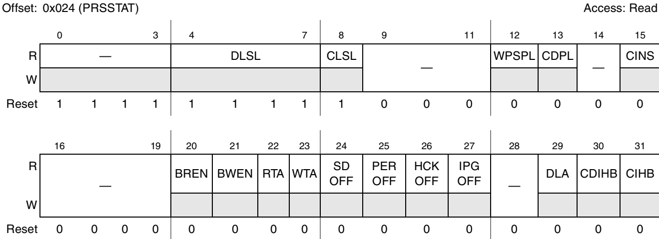
Figure 11-9. Present State Register (PRSTAT)
