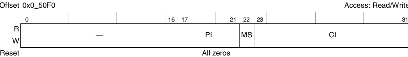
Figure 10-24. Flash Page Address Register, Small Page Device (ORx[PGS] = 0)
