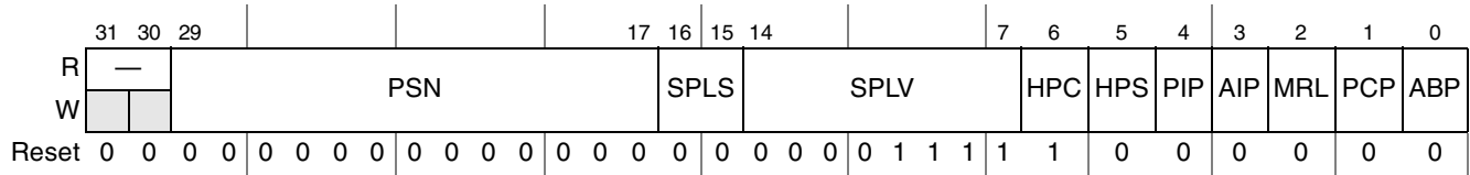
Figure 15-89. PCI Express Slot Capabilities Update Register
