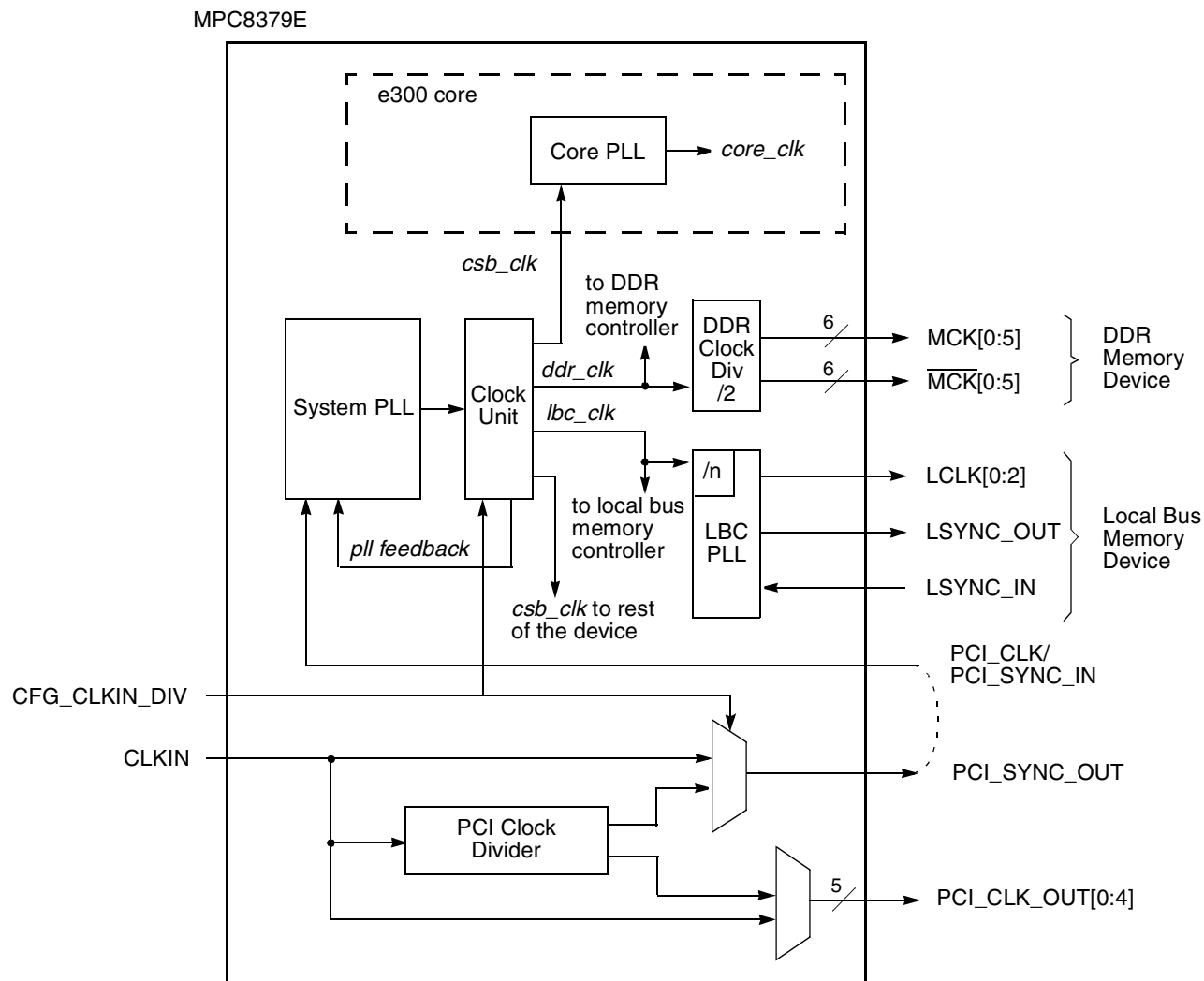
Figure 4-8. Clock Subsystem Block Diagram
