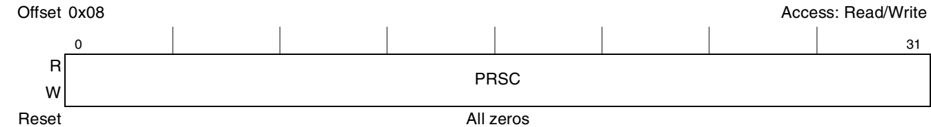
Figure 5-41. Periodic Interval Timer Prescale Register (PTPSR)
