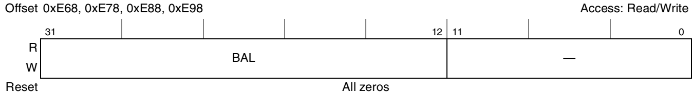
Figure 15-137. PCI Express RC Inbound Window Base Address Register Low n (PEX_RCIWBARL0–PEX_RCIWBARL3)
