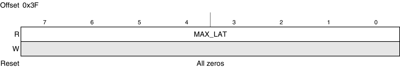
Figure 14-41. Maximum Latency Configuration Register
