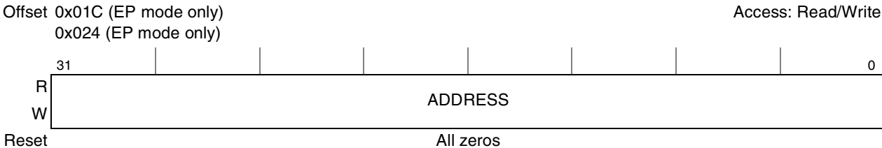
Figure 15-15. 64-Bit High Memory Base Address Registers 3 and 5 (BAR3/BAR5)
