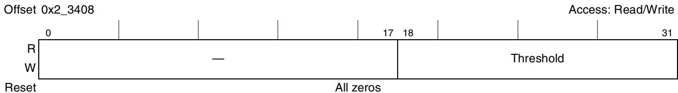
Figure 20-31. Age Count Threshold (AGE_CNT_THRESH)
