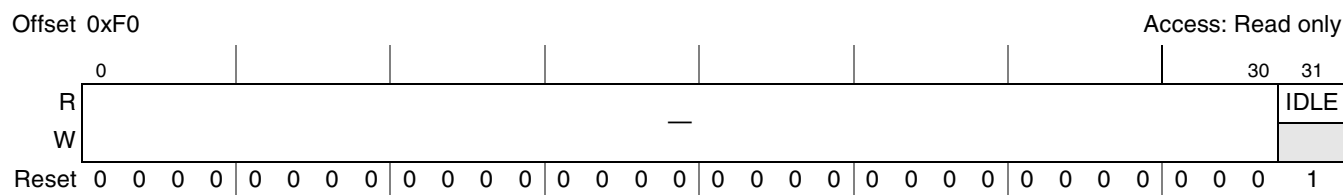
Figure 12-5. Power Management Control Register (PMCR)
