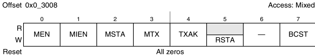
Figure 21-4. I 2 C n Control Register (I2C n CR)
