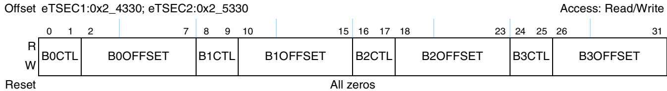
Figure 18-26. RBIFX Register Definition
