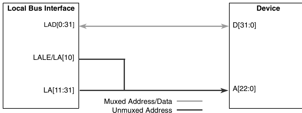
Figure 10-71. Non-Multiplexed Address and Data Buses
