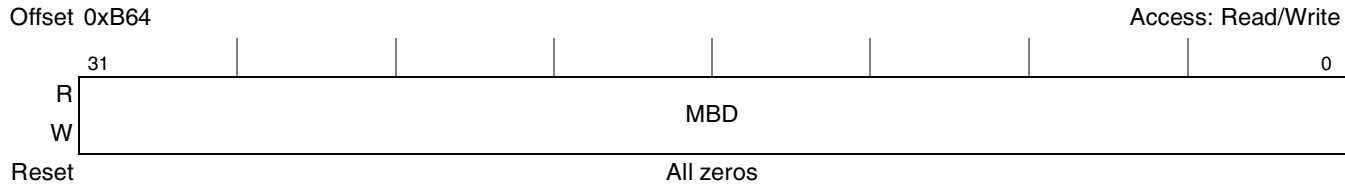
Figure 15-113. PCI Express Inbound Mailbox Data Register (PEX_IMBDR)
