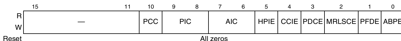
Figure 15-58. PCI Express Slot Control Register
