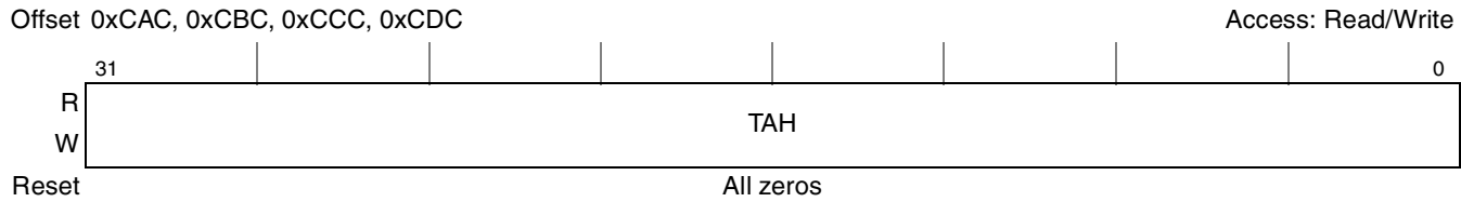
Figure 15-133. PCI Express Outbound Window Translation Address Register High n (PEX_OWTARH0–PEX_OWTARH3)
