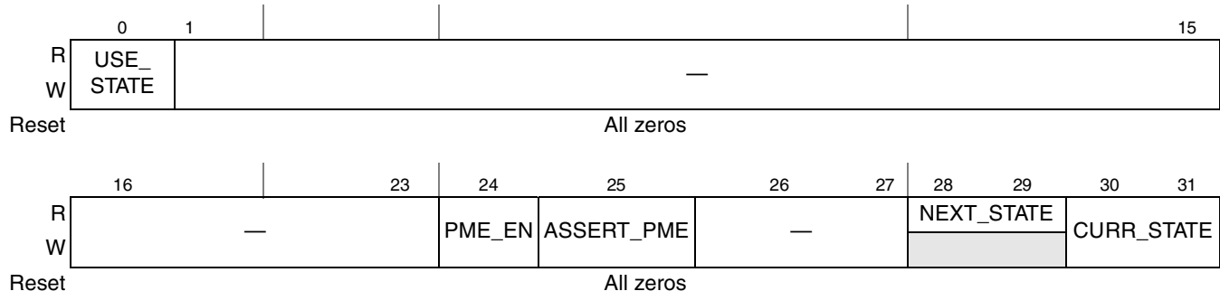
Figure 5-60. Power Management Controller Configuration Register 1
