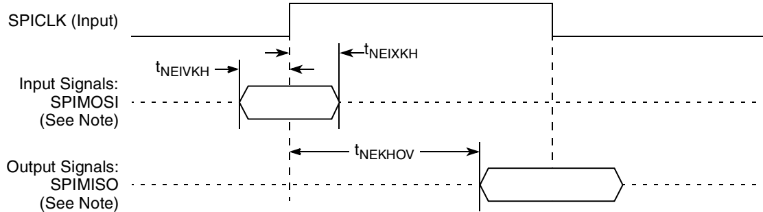
Figure 41. SPI AC Timing in Slave Mode (External Clock) Diagram
