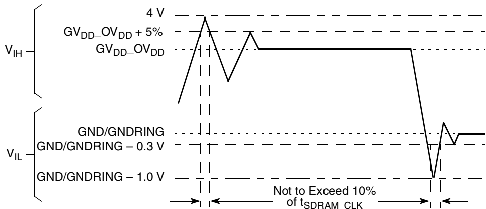
Figure 3. Overshoot/Undershoot Voltage
