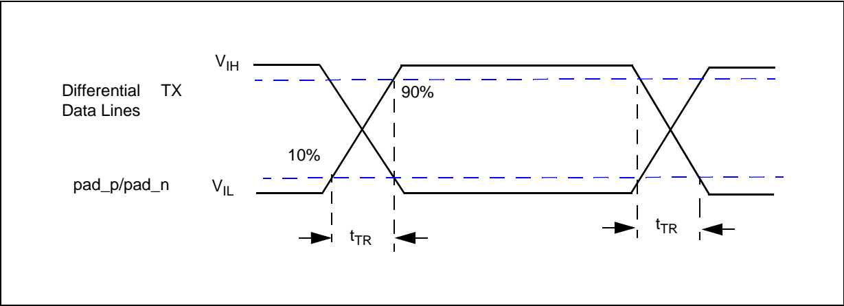
Figure 18. Rise/fall time
